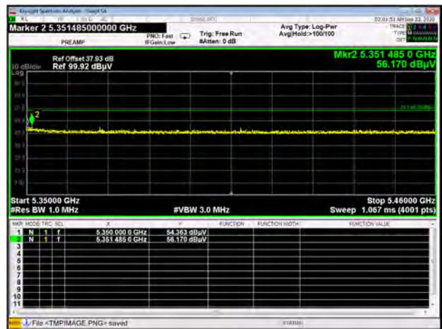
U-NII-2A 11ax20-SU CH64 Peak
