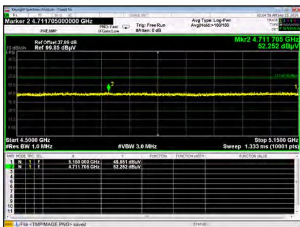
U-NII-2A 11ax40-SU CH54 Peak
