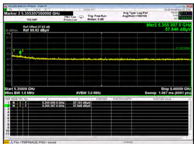
U-NII-2A 11ax40-SU CH62 Peak
