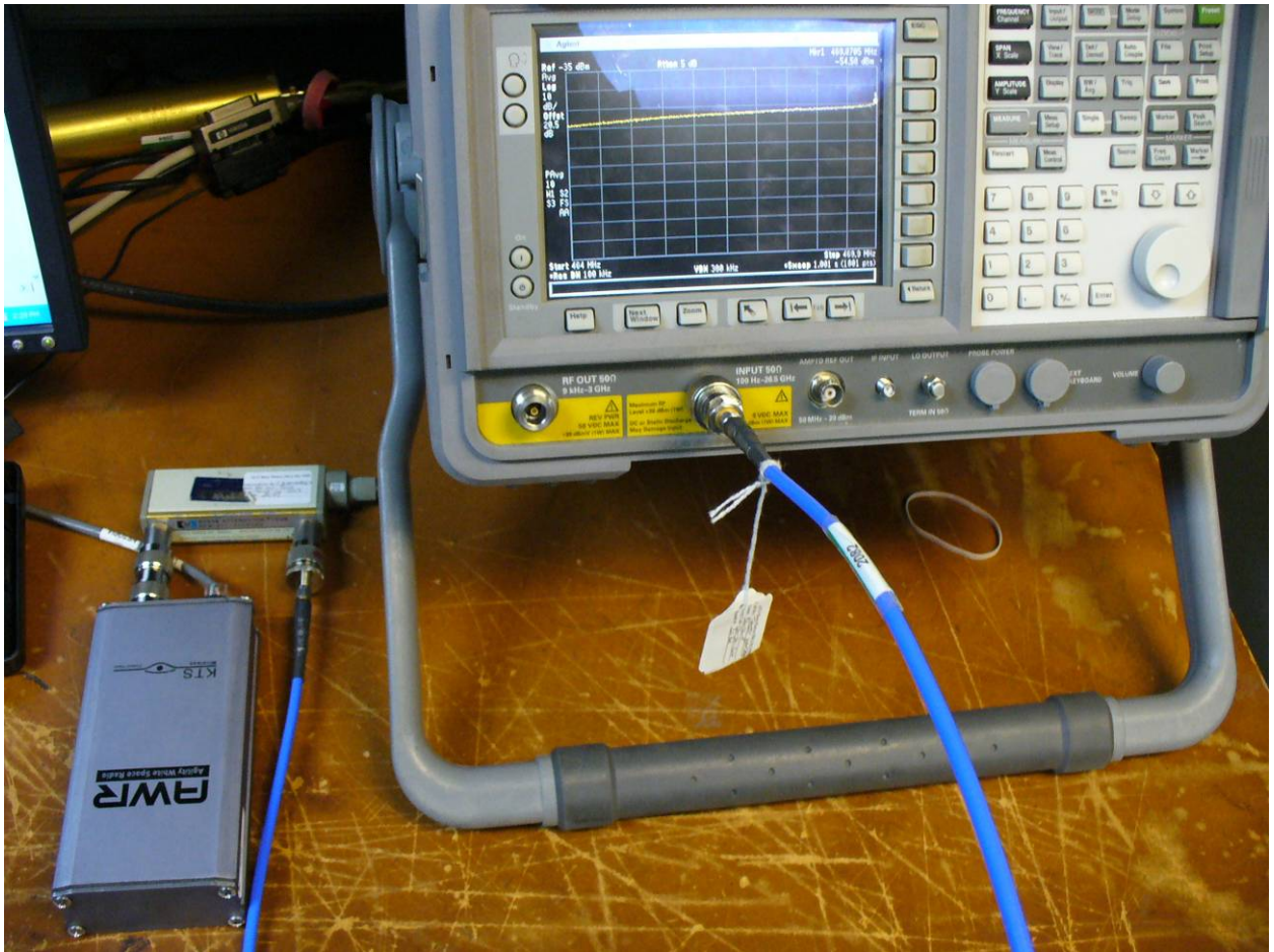
Figure 4: RF Conducted Measurements
