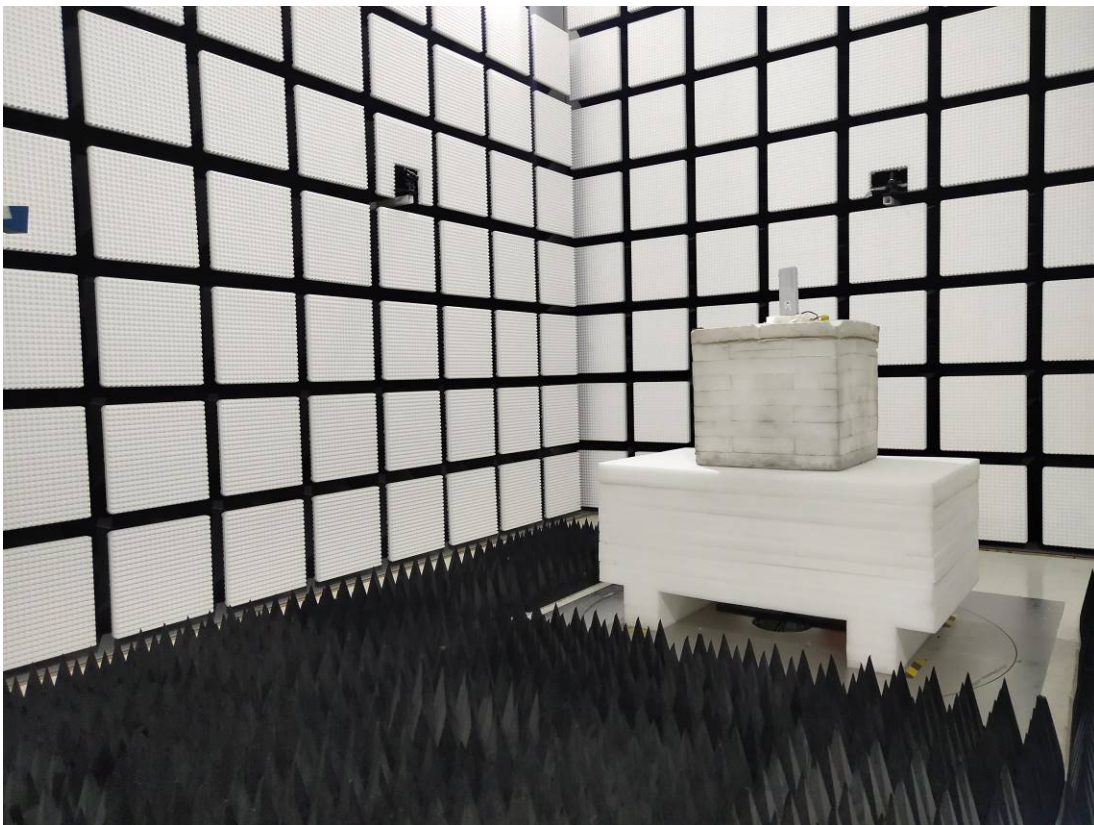
Radiated Emission 18-26.5GHz View POE
