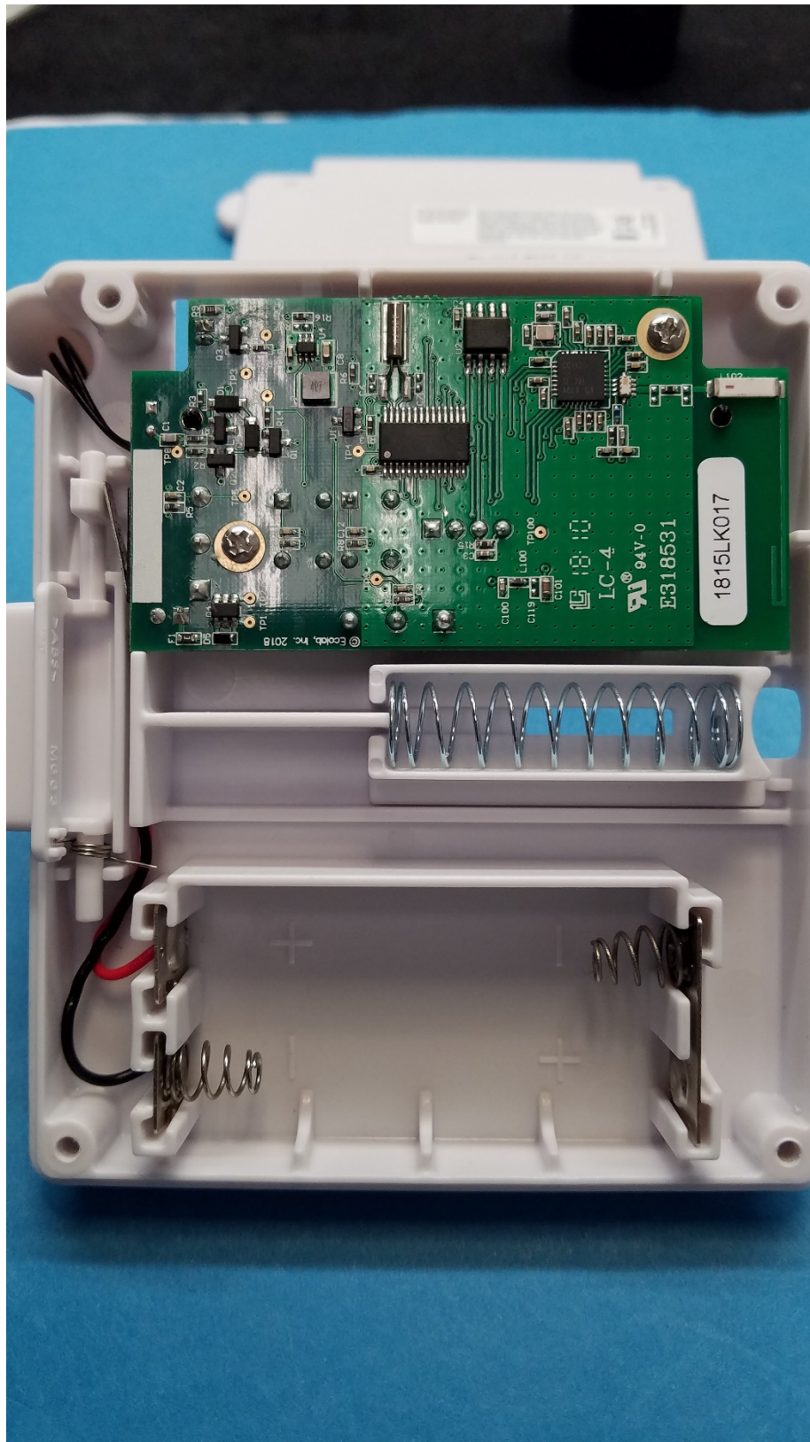
Figure 3: Assembled View
