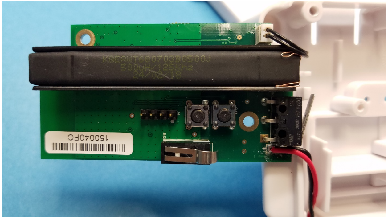
Figure 1: PCB Front
