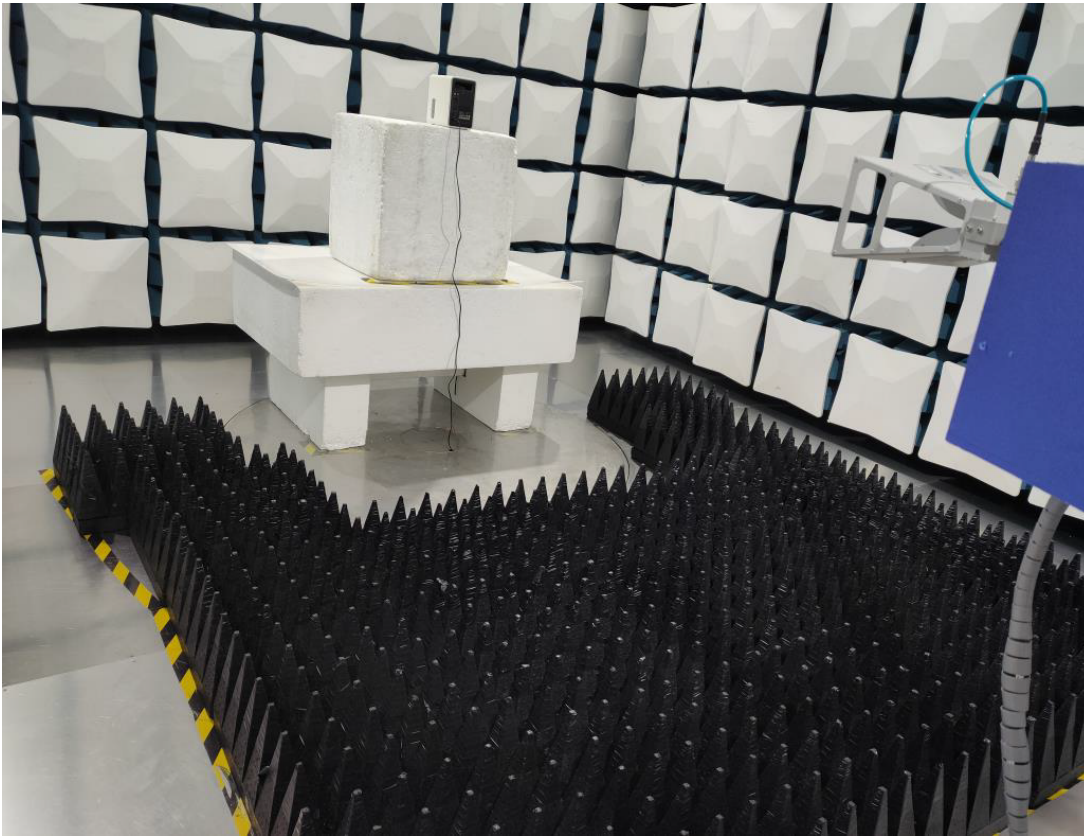
Photograph 3: Set-up for Radiated Spurious Emission, 1GHz - 18GHz
