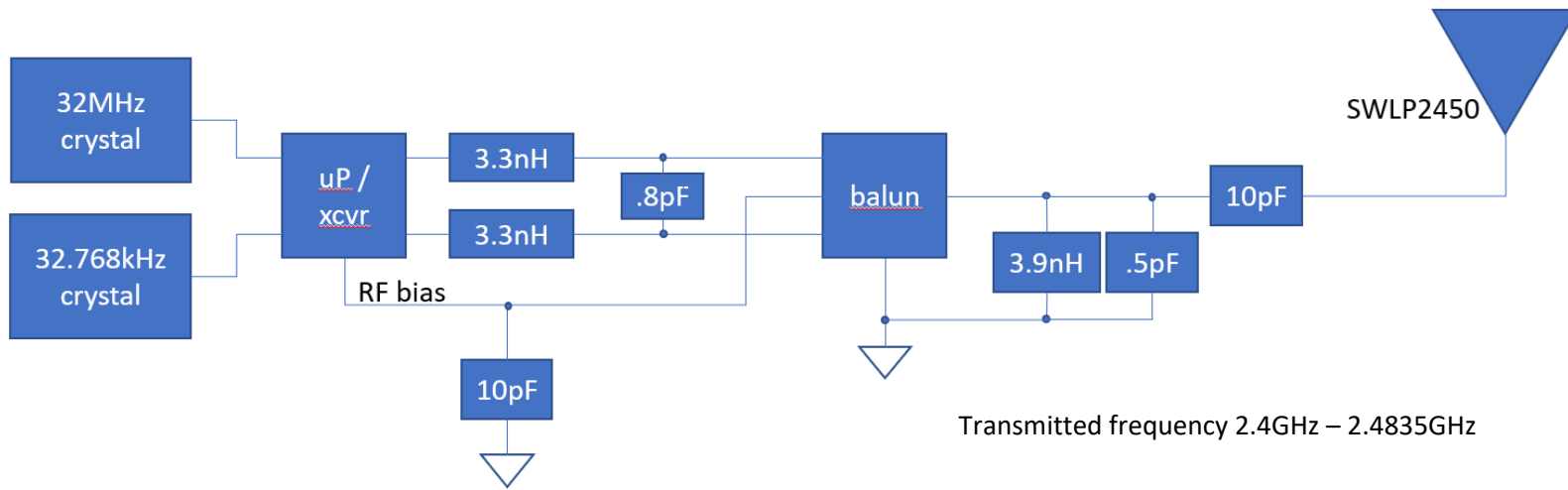
WDS Radio Block Diagram
