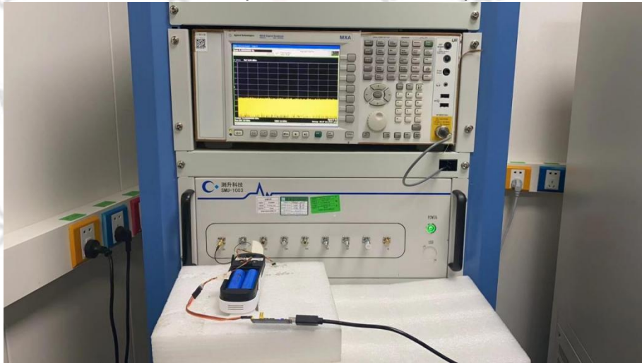
Conducted spurious emission test photos
