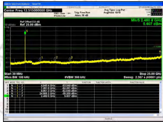
30.0 MHz - 25000.0 MHz
