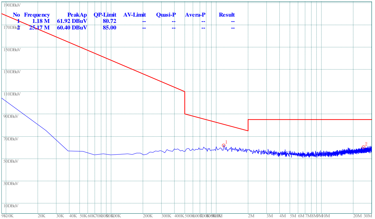
(Plot A.0: 9kHz to 30MHz @ GFSK, channel 0)
