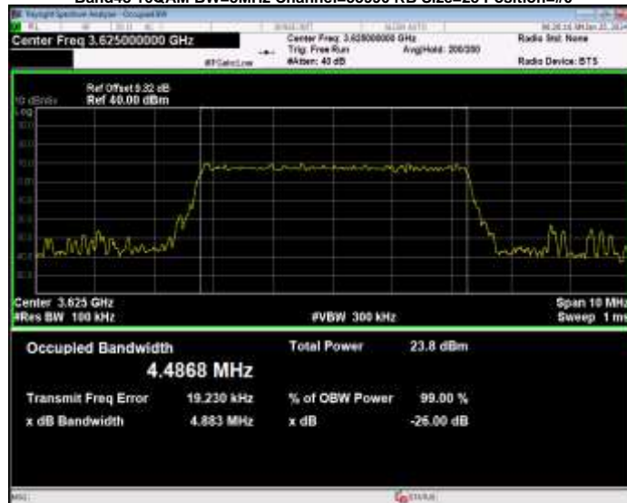
Band48 16QAM BW=5MHz Channel=55990 RB Size=25 Position=#0
