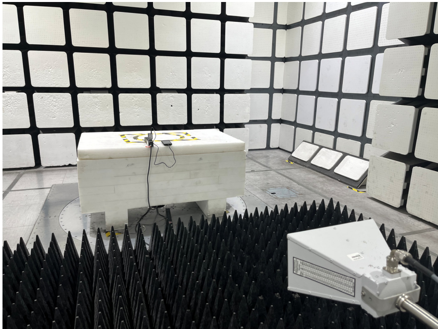
Radiated Emissions Rear View (1-18 GHz)
