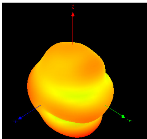
2.4G 3D
