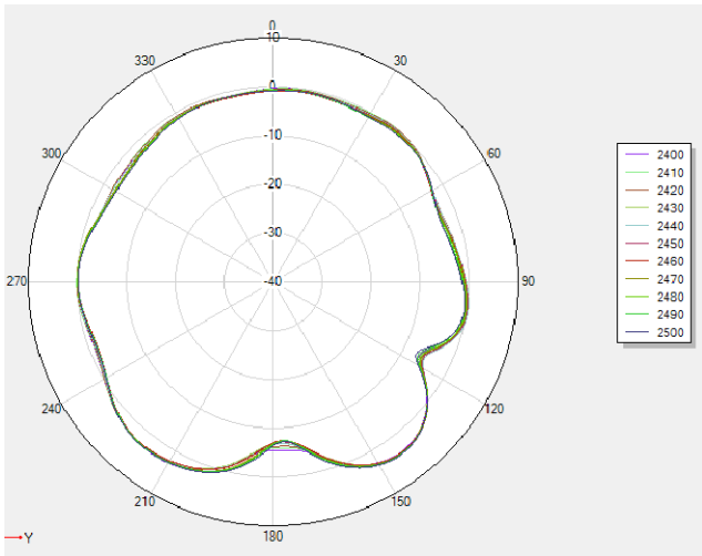
2.4G phi=90deg
