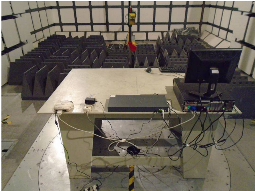
Radiated Emissions Rear View (Below 1 GHz, Power by adapter)
