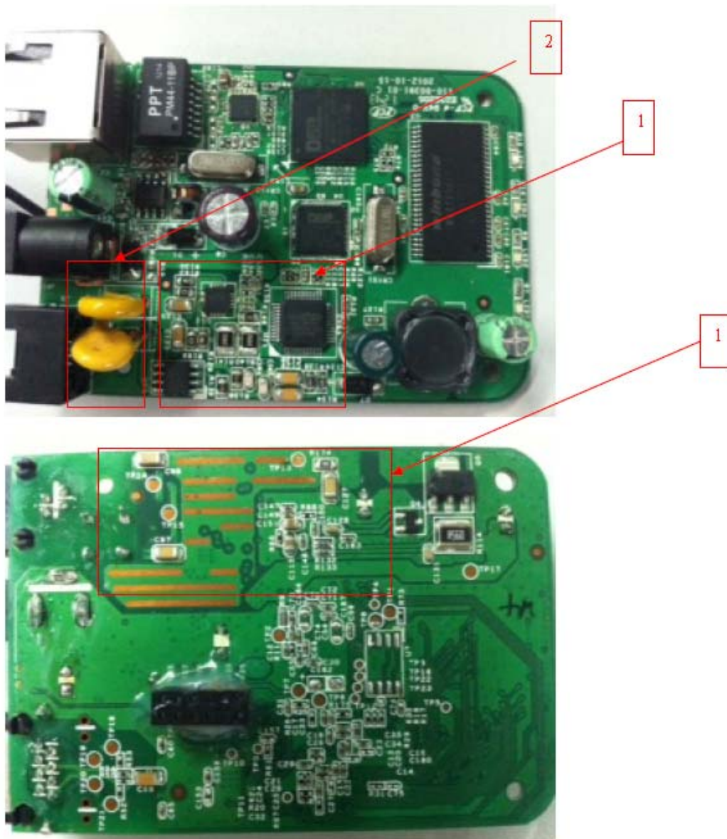
Original mainboard photo view
