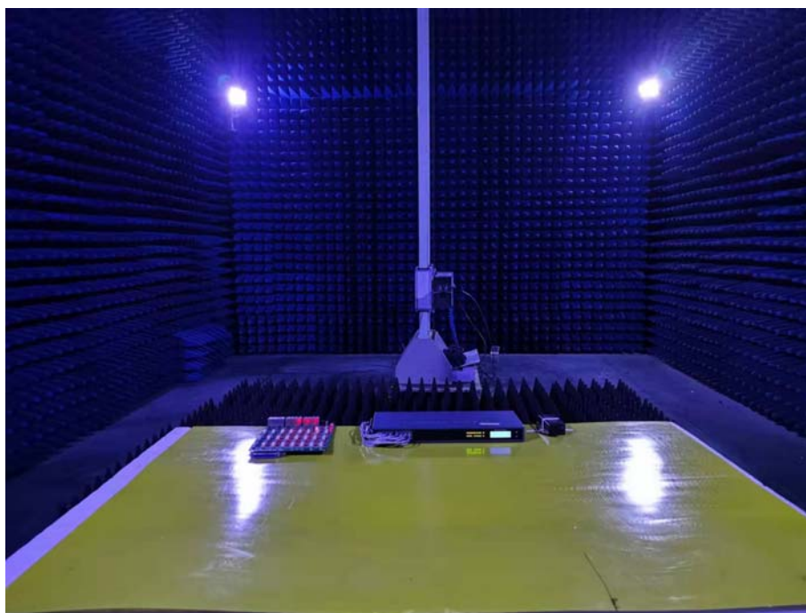
Photo of Radiated Emission Measurement (Above 1G) Test Mode 1: Full Load (RJ11)
