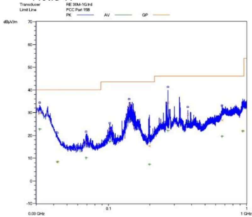
Horizontal: Radiated Emission Test Plot -(30-1000MHz)
