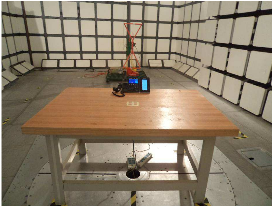
Radiated Emissions - Front View (Powered by PoE)
