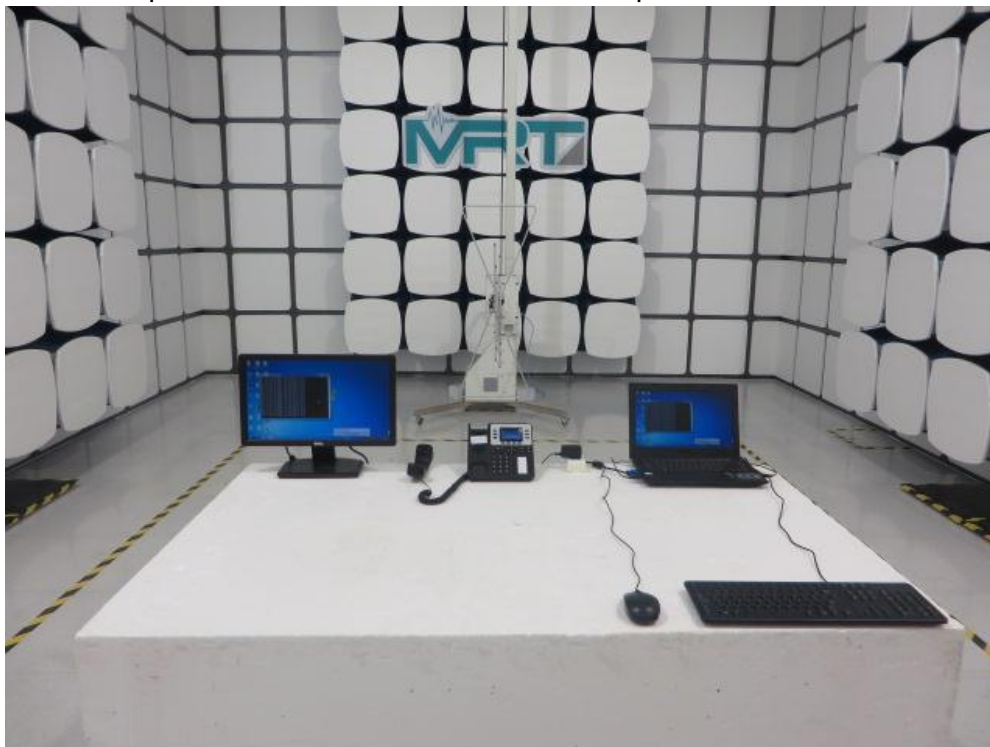
Description: Radiated disturbance Test Setup for 30MHz ~ 1GHz
