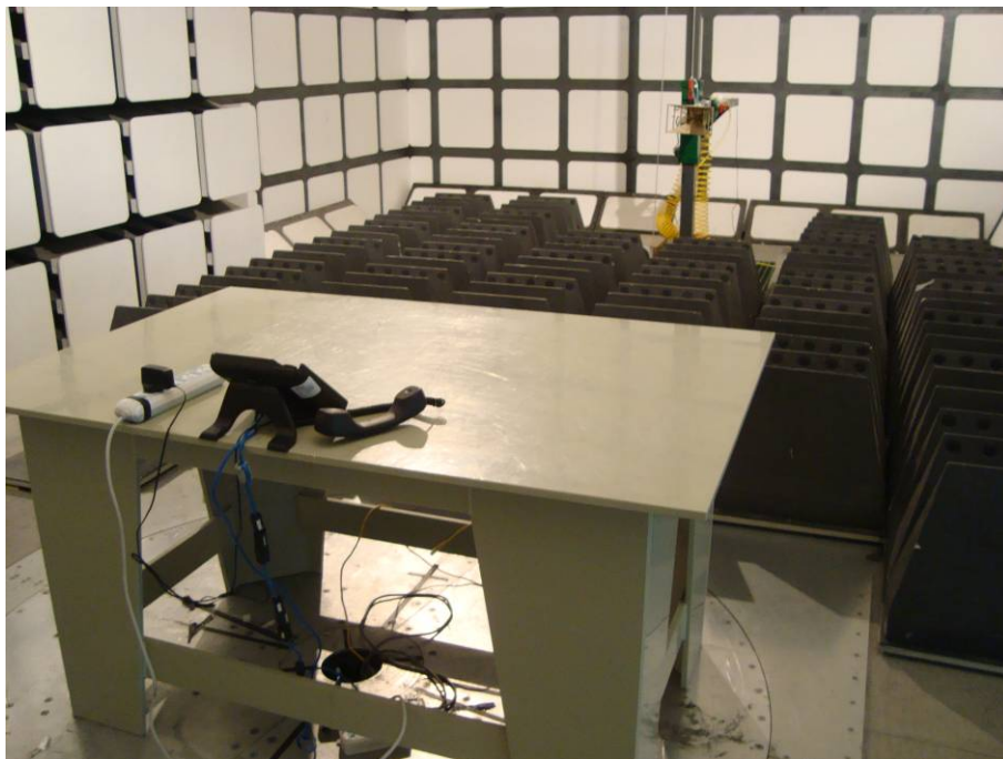
Radiated Emissions - Rear View (Above 1 GHz, Powered by AC/DC adapter)
