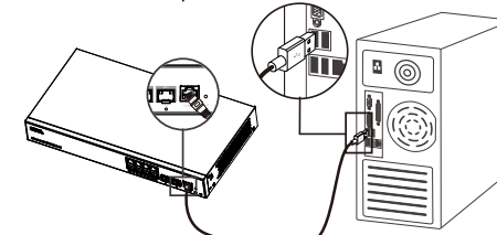
Connect to Console Port (USB)
