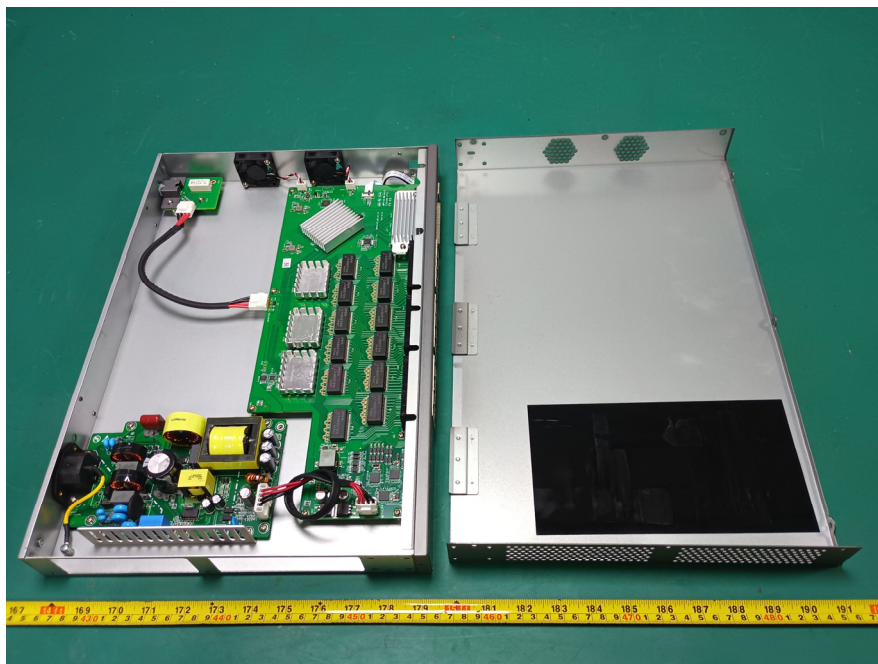
Power Supply(G1766-0400W)
