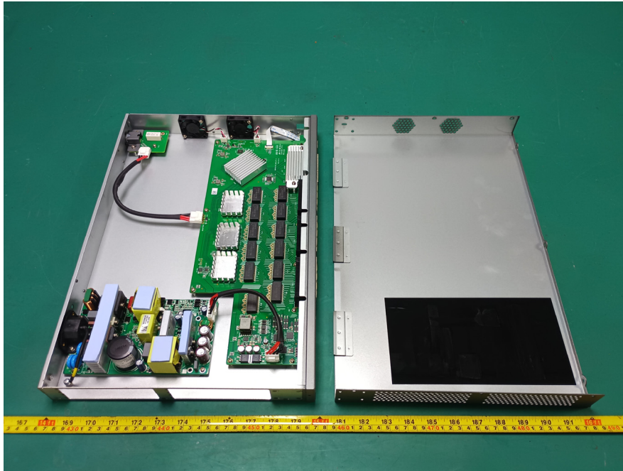
Power Supply(D1602-F420S54-A)
