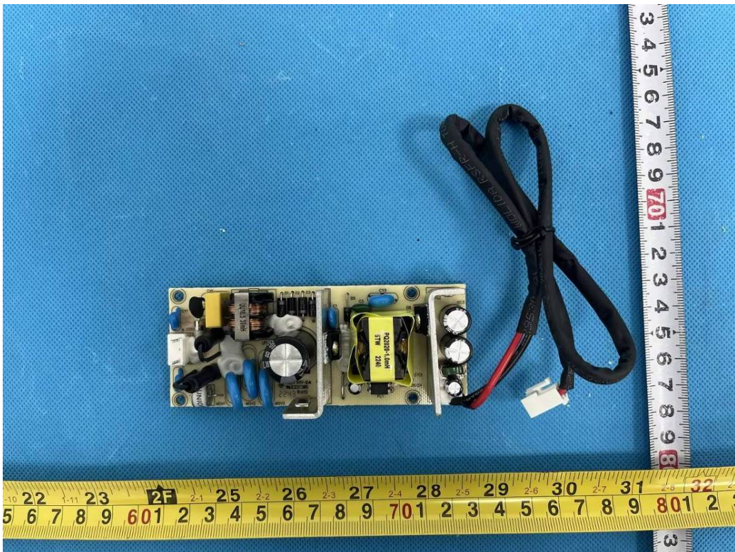
Power #1: R0001B(RB030W05-1302300)
