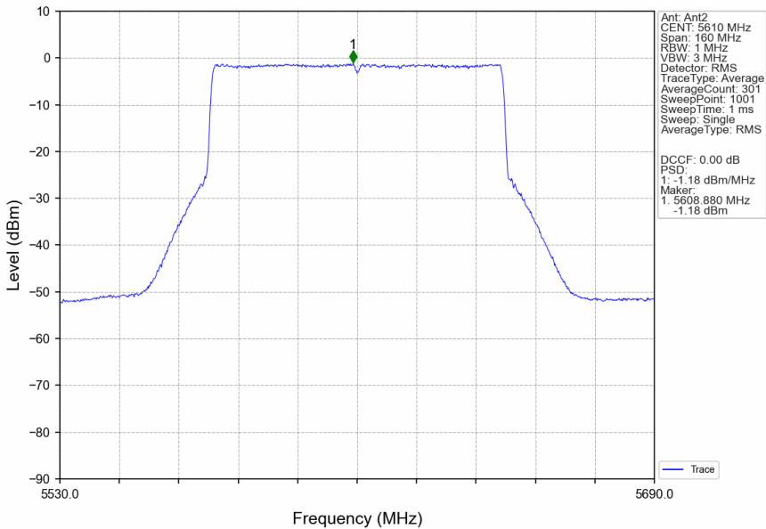
802.11ax(HEW80)_HCH_5610MHz_SU_/_Ant2_NTNV
