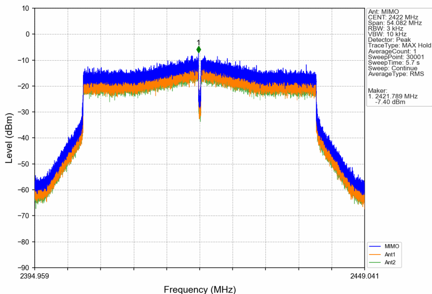
802.11ax(HEW40)_LCH_2422MHz_RU484_Left_MIMO_NTNV
