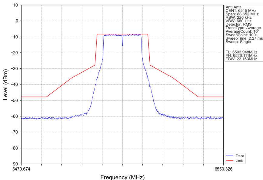
802.11a_HCH_6515MHz_Ant1_NTNV
