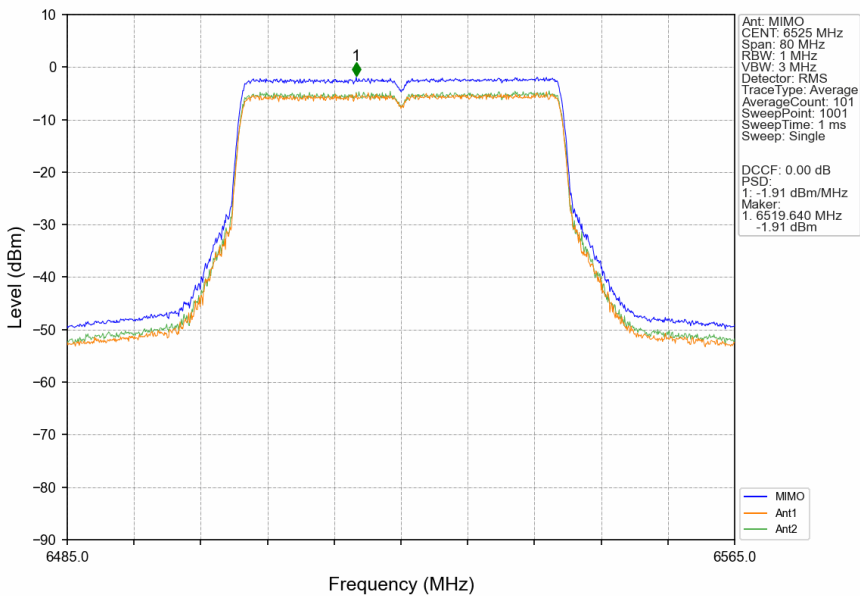
802.11ax(HEW40)_HCH_6525MHz_RU484_Left_MIMO_NTNV
