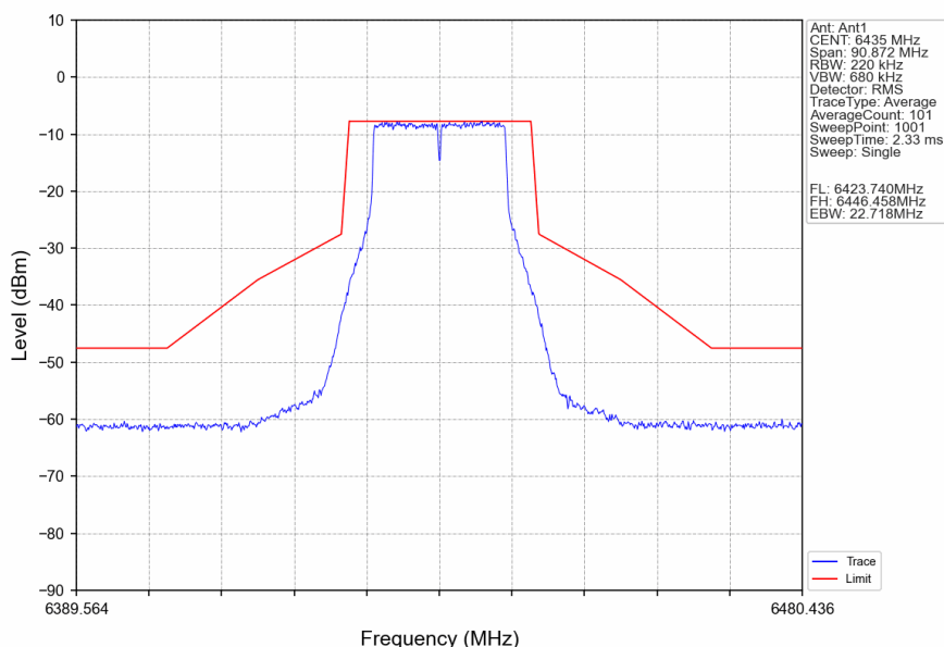
802.11a_LCH_6435MHz_Ant1_NTNV
