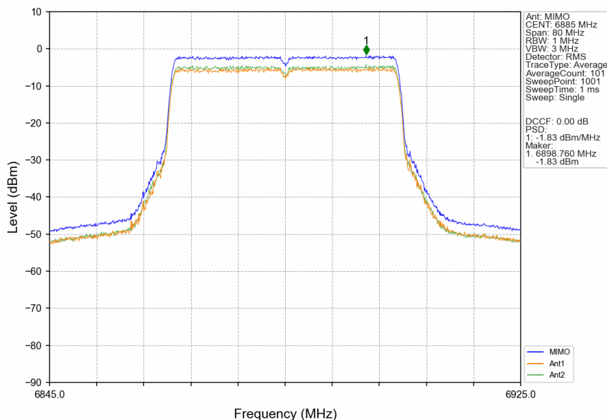
802.11ax(HEW40)_HCH_6885MHz_RU484_Left_MIMO_NTNV
