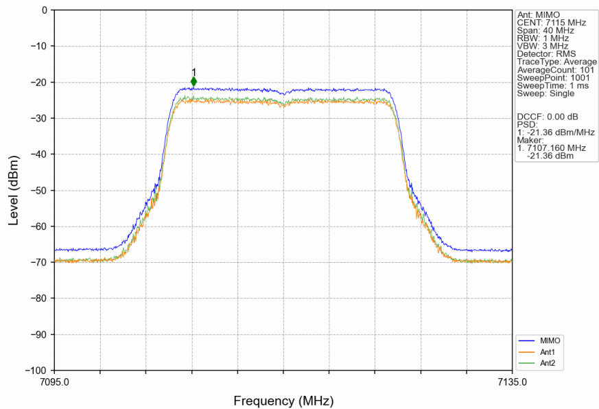
802.11ax(HEW20)_HCH_7115MHz_RU242_Left_MIMO_NTNV
