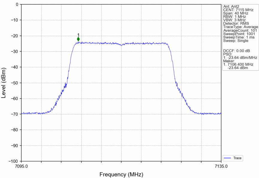
802.11ax(HEW20)_HCH_7115MHz_RU242_Left_Ant2_NTNV
