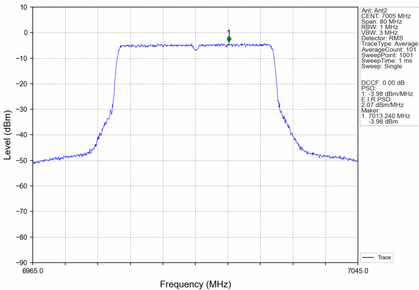
802.11ax(HEW40)_MCH_7005MHz_RU484_Left_Ant2_NTNV
