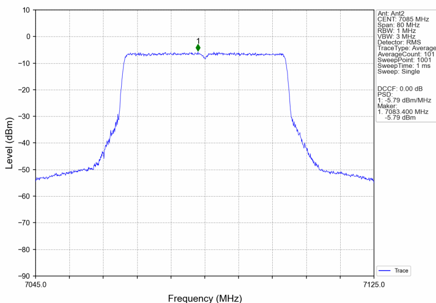
802.11ax(HEW40)_HCH_7085MHz_RU484_Left_Ant2_NTNV
