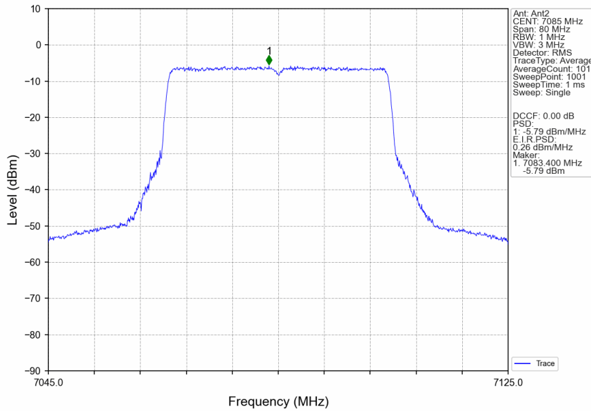
802.11ax(HEW40)_HCH_7085MHz_RU484_Left_Ant2_NTNV
