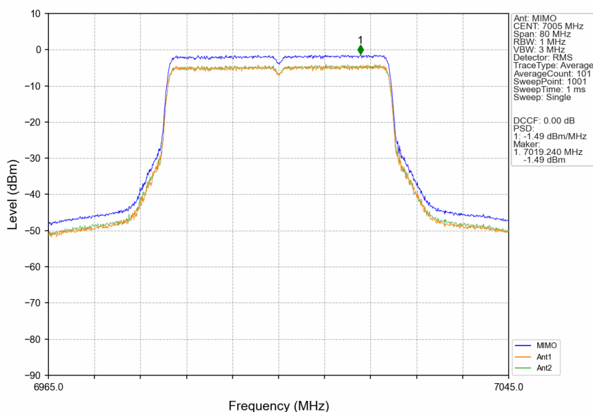
802.11ax(HEW40)_MCH_7005MHz_RU484_Left_MIMO_NTNV
