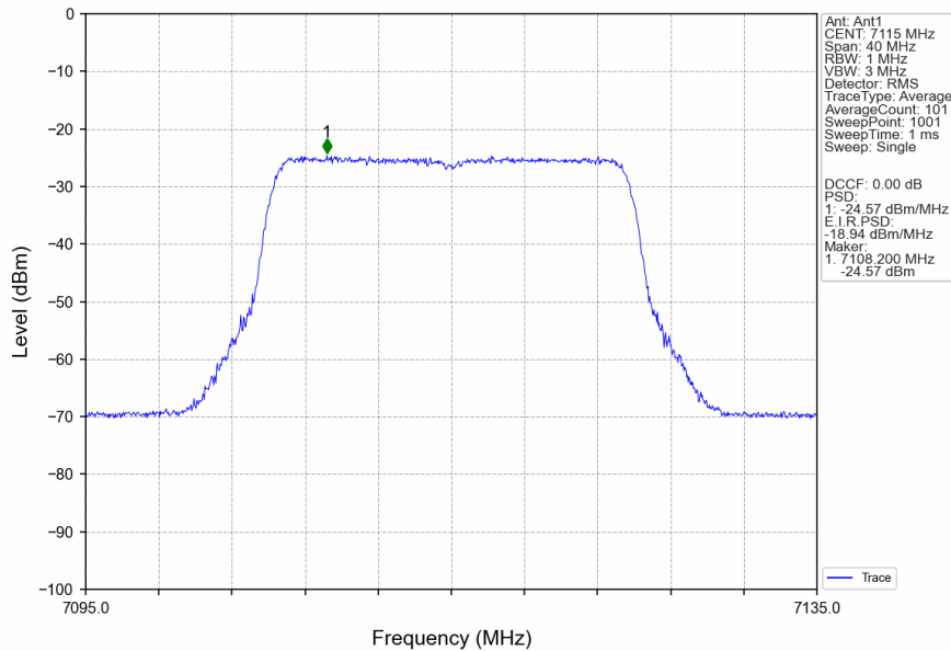
802.11ax(HEW20)_HCH_7115MHz_RU242_Left_Ant1_NTNV
