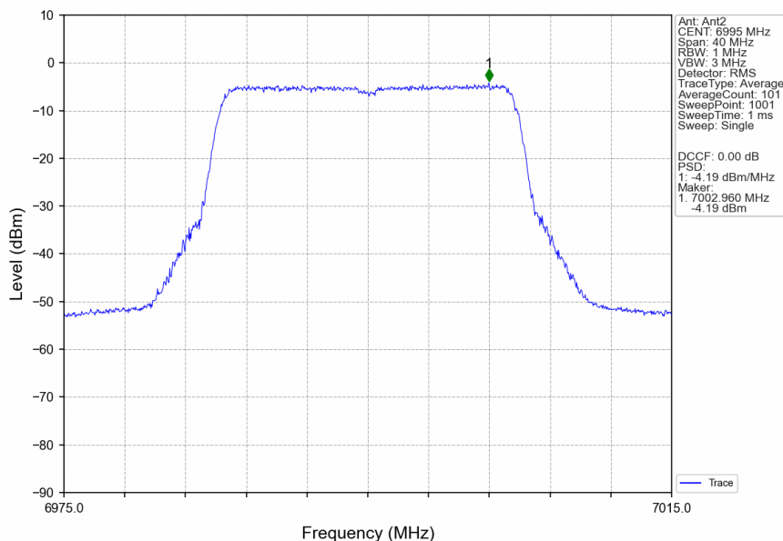
802.11ax(HEW20)_MCH_6995MHz_RU242_Left_Ant2_NTNV
