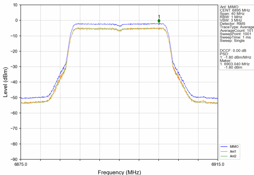
802.11ax(HEW20)_LCH_6895MHz_RU242_Left_MIMO_NTNV
