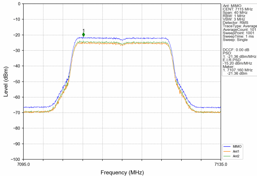
802.11ax(HEW20)_HCH_7115MHz_RU242_Left_MIMO_NTNV
