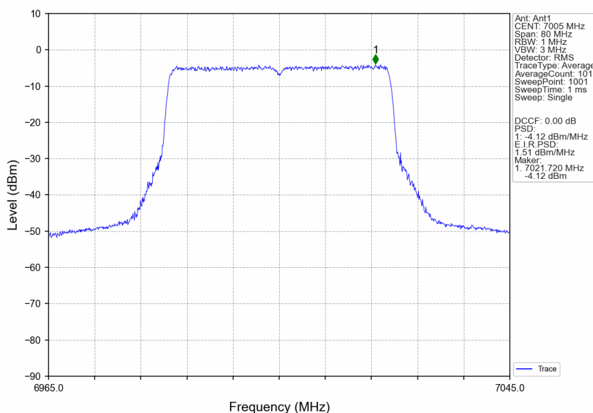
802.11ax(HEW40)_MCH_7005MHz_RU484_Left_Ant1_NTNV
