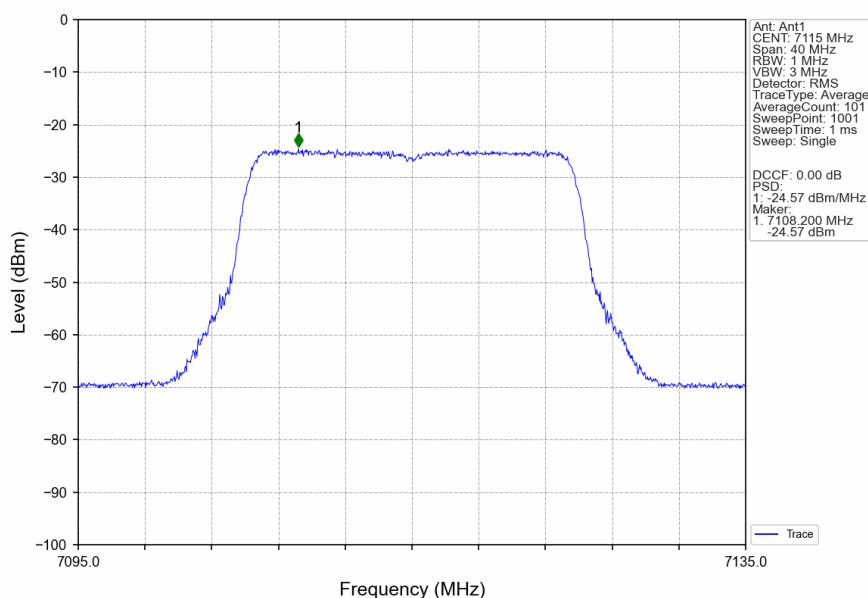
802.11ax(HEW20)_HCH_7115MHz_RU242_Left_Ant1_NTNV
