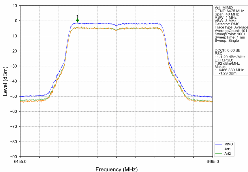
802.11ax(HEW20)_MCH_6475MHz_RU242_Left_MIMO_NTNV
