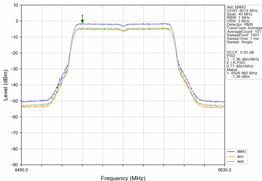
802.11ax(HEW20)_HCH_6515MHz_RU242_Left_MIMO_NTNV
