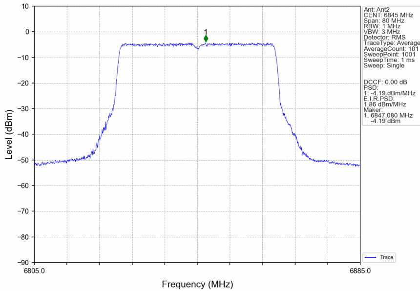
802.11ax(HEW40)_HCH_6845MHz_RU484_Left_Ant2_NTNV
