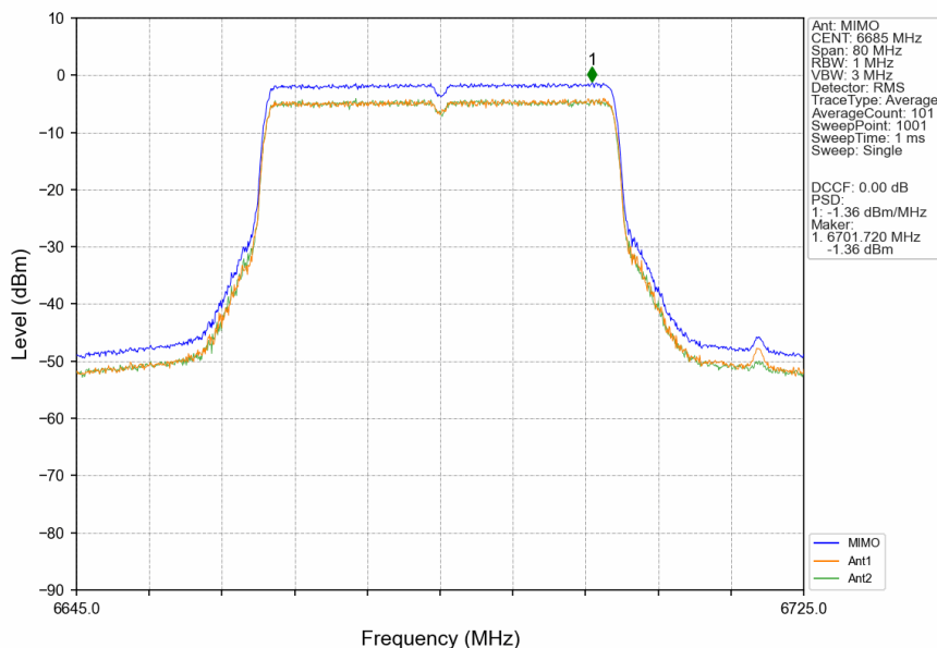
802.11ax(HEW40)_MCH_6685MHz_RU484_Left_MIMO_NTNV
