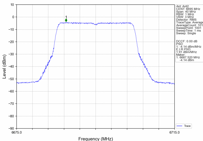
802.11ax(HEW20)_MCH_6695MHz_RU242_Left_Ant2_NTNV
