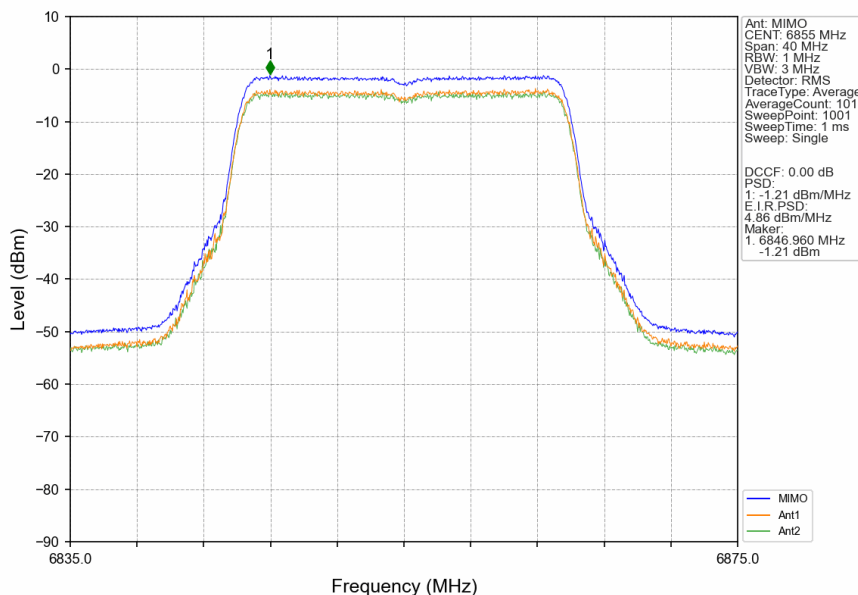
802.11ax(HEW20)_HCH_6855MHz_RU242_Left_MIMO_NTNV
