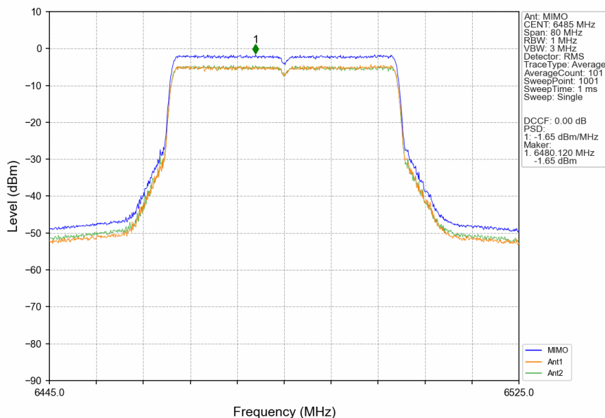
802.11ax(HEW40)_MCH_6485MHz_RU484_Left_MIMO_NTNV
