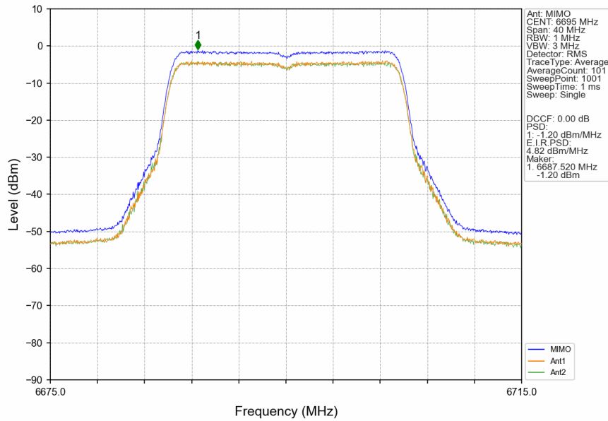
802.11ax(HEW20)_MCH_6695MHz_RU242_Left_MIMO_NTNV
