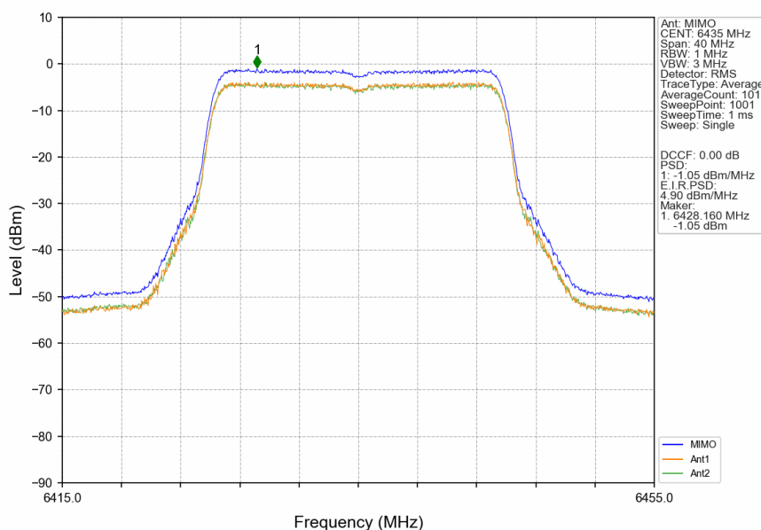
802.11ax(HEW20)_LCH_6435MHz_RU242_Left_MIMO_NTNV
