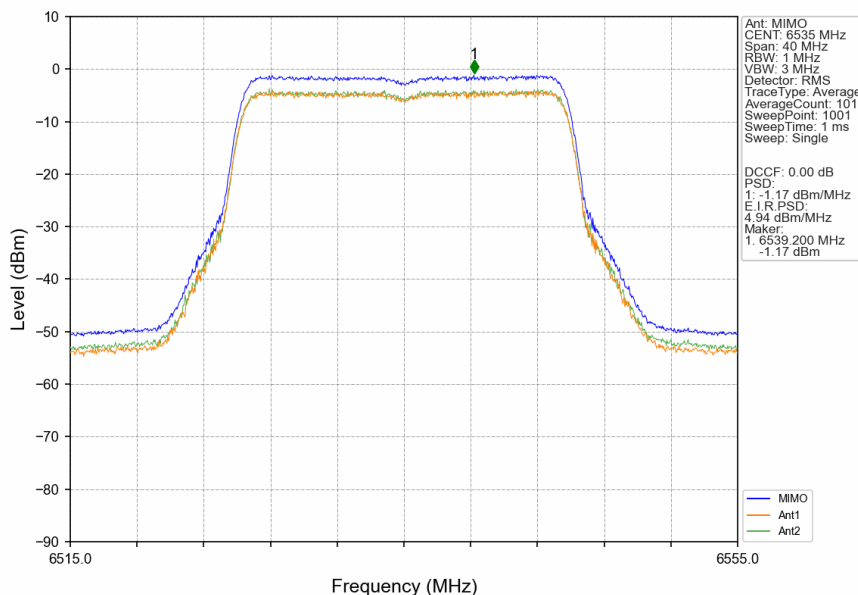
802.11ax(HEW20)_LCH_6535MHz_RU242_Left_MIMO_NTNV
