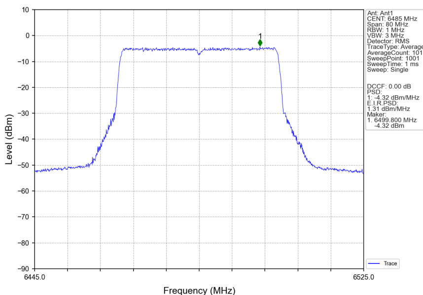
802.11ax(HEW40)_MCH_6485MHz_RU484_Left_Ant1_NTNV
