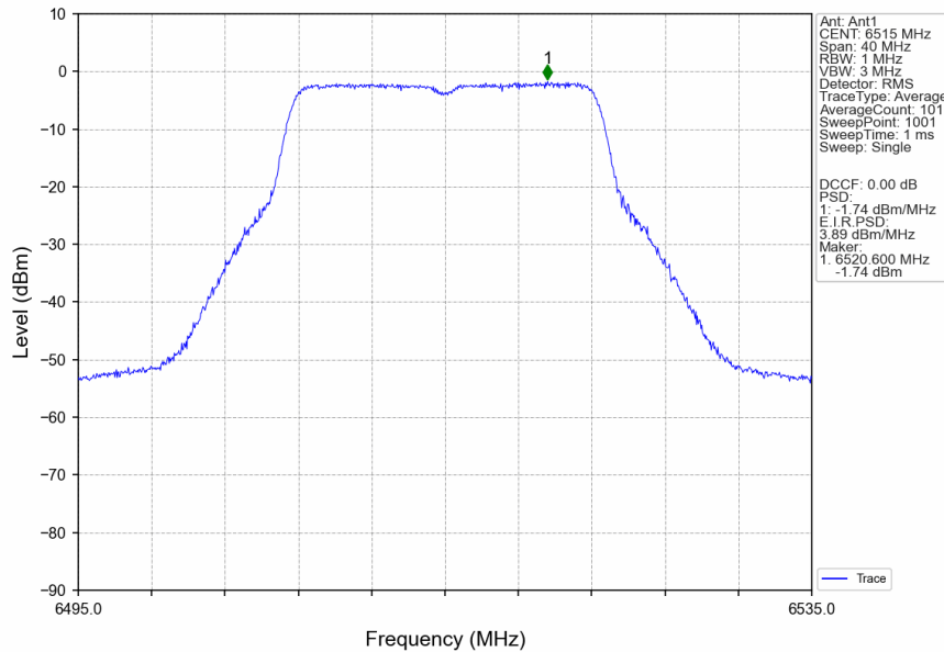
802.11a_HCH_6515MHz_Ant1_NTNV
