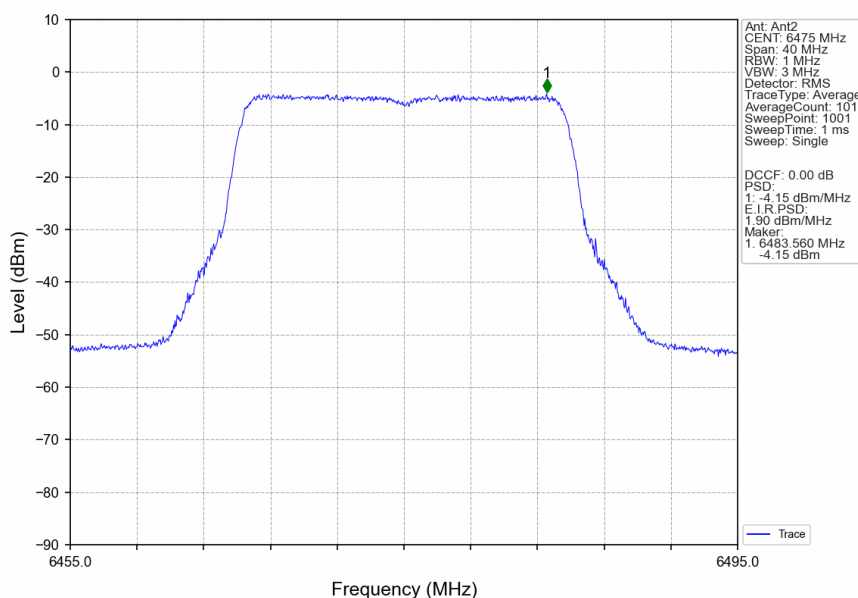
802.11ax(HEW20)_MCH_6475MHz_RU242_Left_Ant2_NTNV
