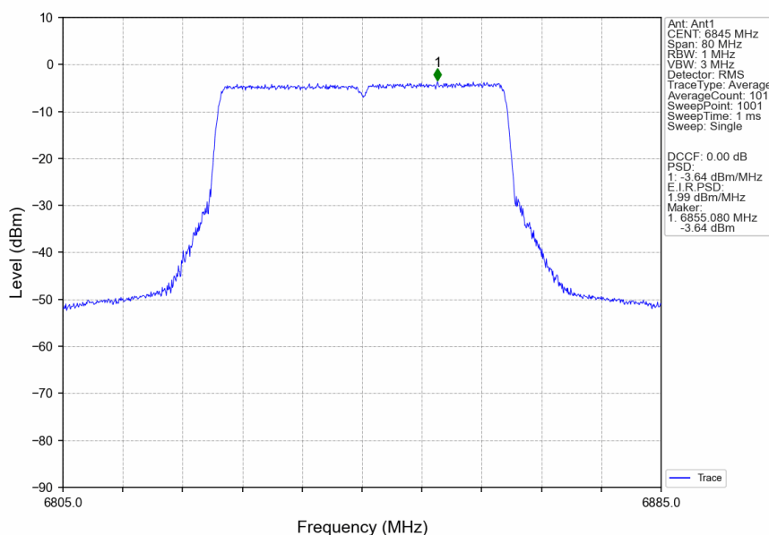
802.11ax(HEW40)_HCH_6845MHz_RU484_Left_Ant1_NTNV
