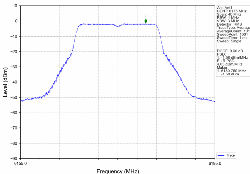
802.11a_MCH_6175MHz_Ant1_NTNV
