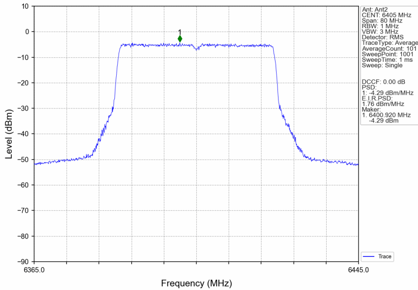
802.11ax(HEW40)_HCH_6405MHz_RU484_Left_Ant2_NTNV
