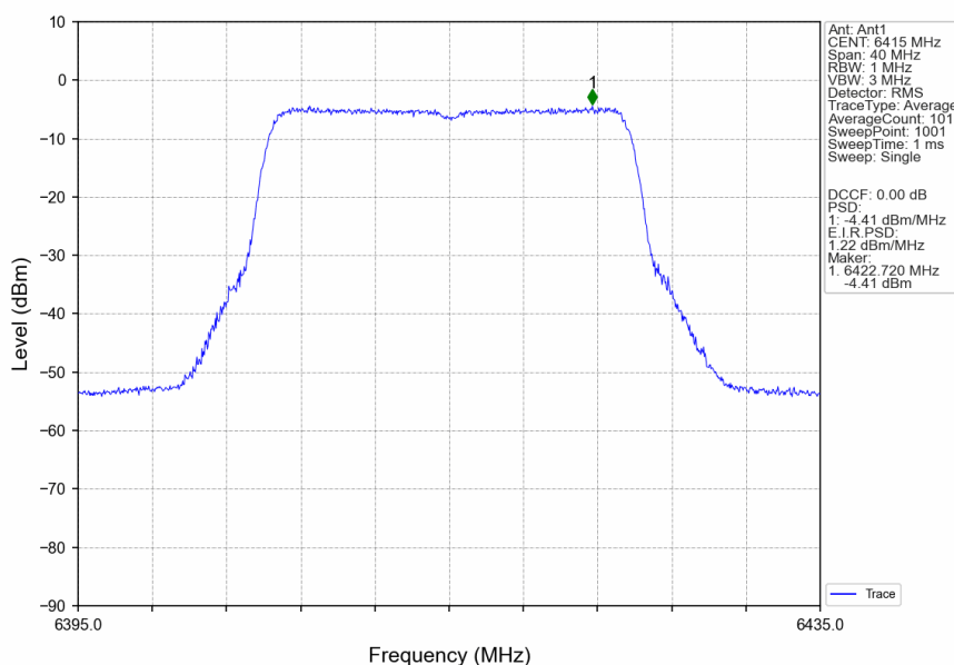
802.11ax(HEW20)_HCH_6415MHz_RU242_Left_Ant1_NTNV
