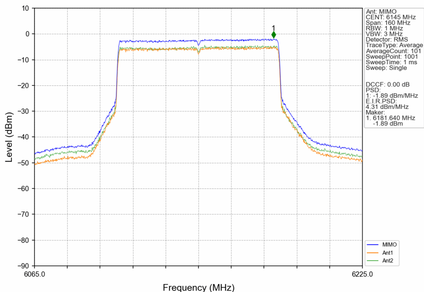
802.11ax(HEW80)_MCH_6145MHz_RU996_Left_MIMO_NTNV
