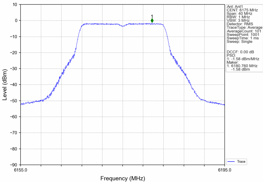
802.11a_MCH_6175MHz_Ant1_NTNV
