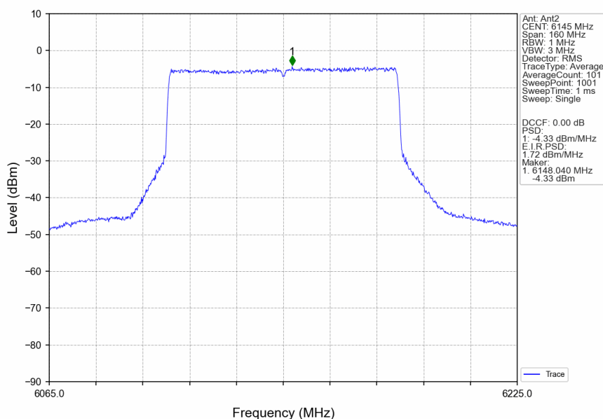
802.11ax(HEW80)_MCH_6145MHz_RU996_Left_Ant2_NTNV
