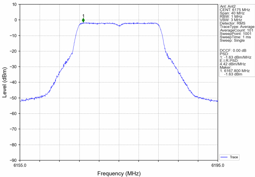
802.11a_MCH_6175MHz_Ant2_NTNV
