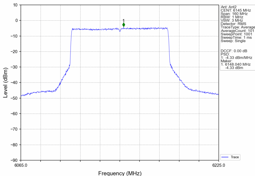
802.11ax(HEW80)_MCH_6145MHz_RU996_Left_Ant2_NTNV
