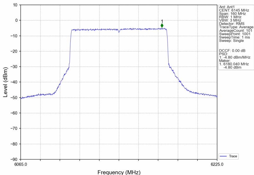
802.11ax(HEW80)_MCH_6145MHz_RU996_Left_Ant1_NTNV
