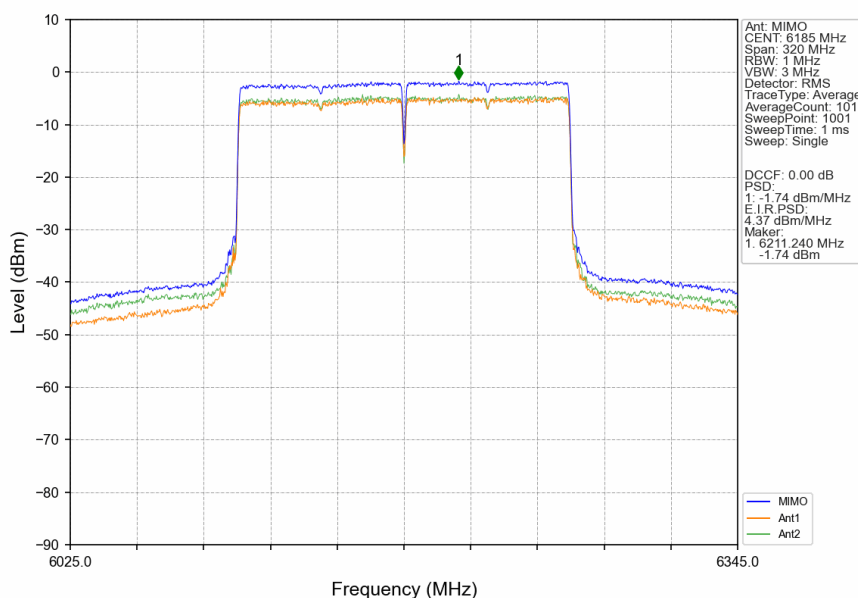
802.11ax(HEW160)_MCH_6185MHz_2xRU996_Left_MIMO_NTNV
