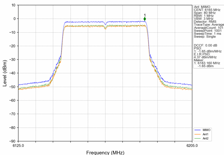
802.11ax(HEW40)_MCH_6165MHz_RU484_Left_MIMO_NTNV
