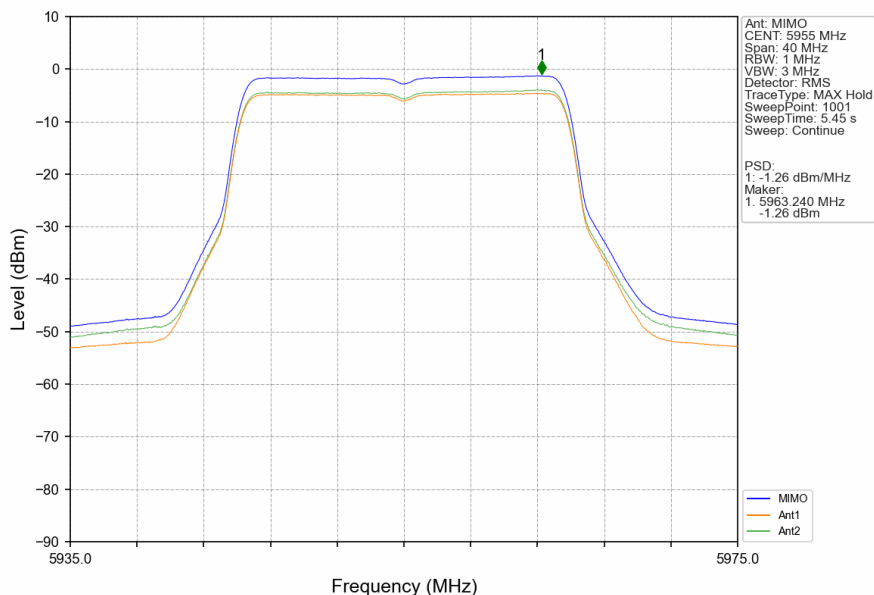
802.11ax(HEW20)_LCH_5955MHz_RU242_Left_MIMO_NTNV
