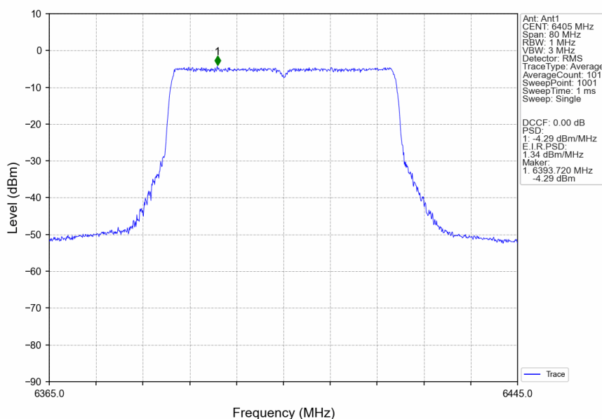
802.11ax(HEW40)_HCH_6405MHz_RU484_Left_Ant1_NTNV
