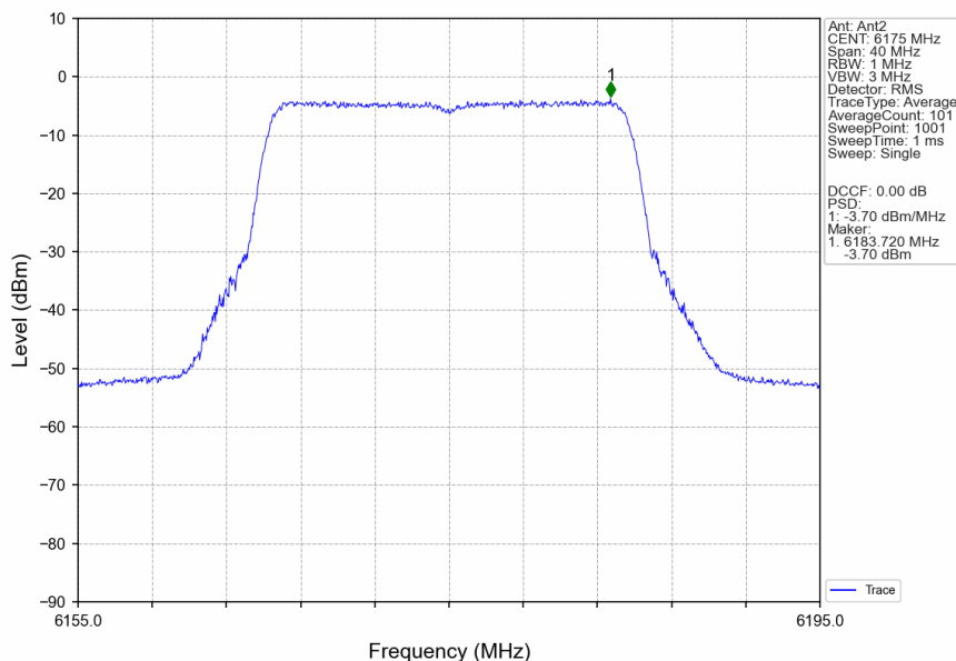
802.11ax(HEW20)_MCH_6175MHz_RU242_Left_Ant2_NTNV
