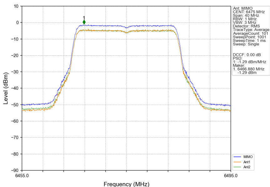
802.11ax(HEW20)_MCH_6475MHz_RU242_Left_MIMO_NTNV
