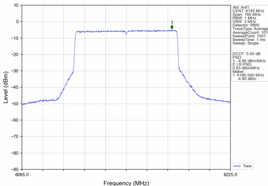
802.11ax(HEW80)_MCH_6145MHz_RU996_Left_Ant1_NTNV
