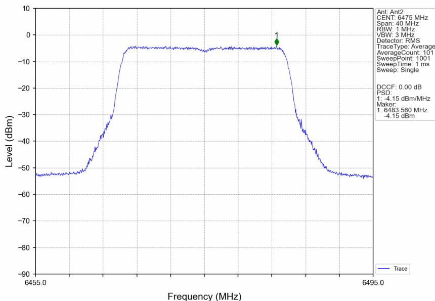
802.11ax(HEW20)_MCH_6475MHz_RU242_Left_Ant2_NTNV
