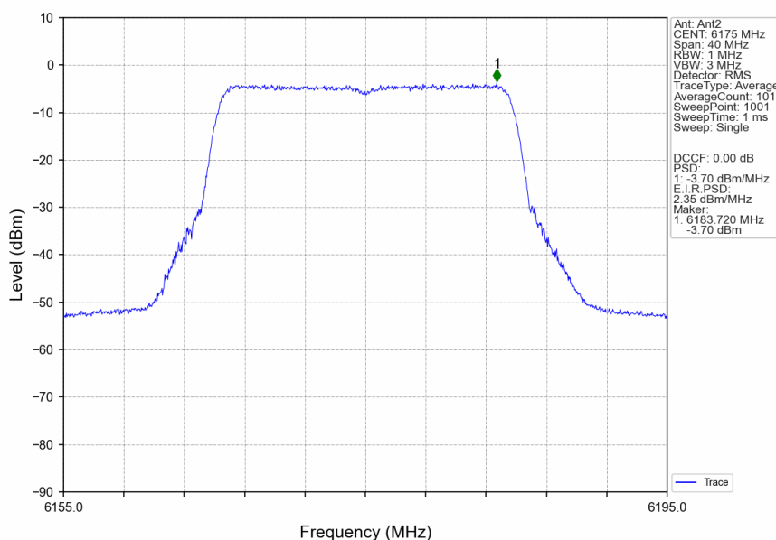
802.11ax(HEW20)_MCH_6175MHz_RU242_Left_Ant2_NTNV
