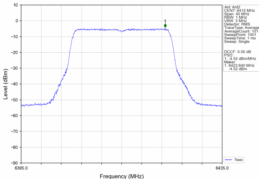
802.11ax(HEW20)_HCH_6415MHz_RU242_Left_Ant2_NTNV
