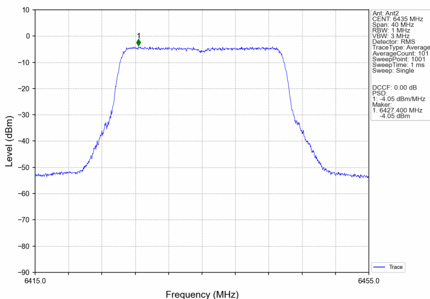
802.11ax(HEW20)_LCH_6435MHz_RU242_Left_Ant2_NTNV
