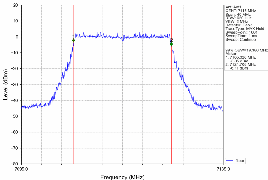
802.11ax(HEW20)_HCH_7115MHz_RU242_Left_Ant1_NTNV
