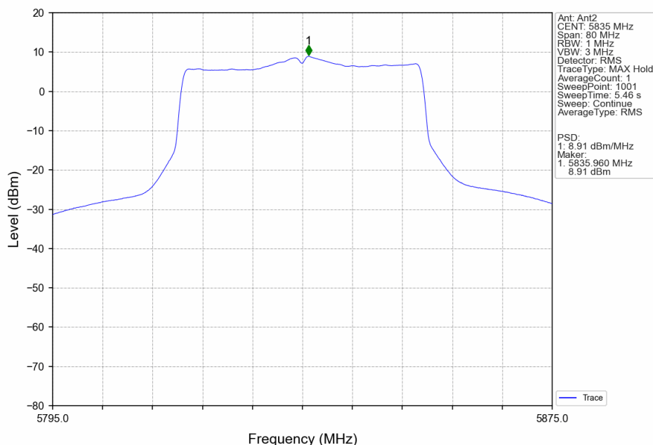
802.11ax(HEW40)_HCH_5835MHz_SU_ / _MIMO_NTNV
