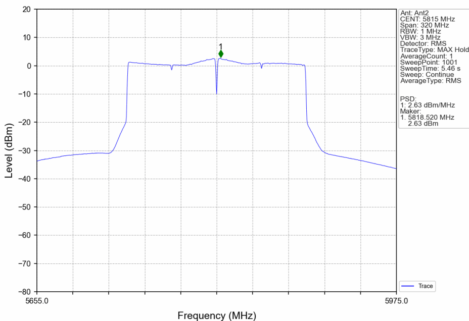
802.11ax(HEW160)_HCH_5815MHz_SU_ / _MIMO_NTNV
