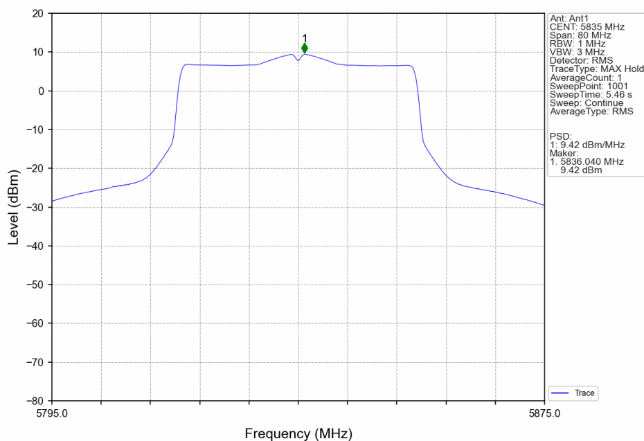
802.11ax(HEW40)_HCH_5835MHz_SU_/_Ant1_NTNV
