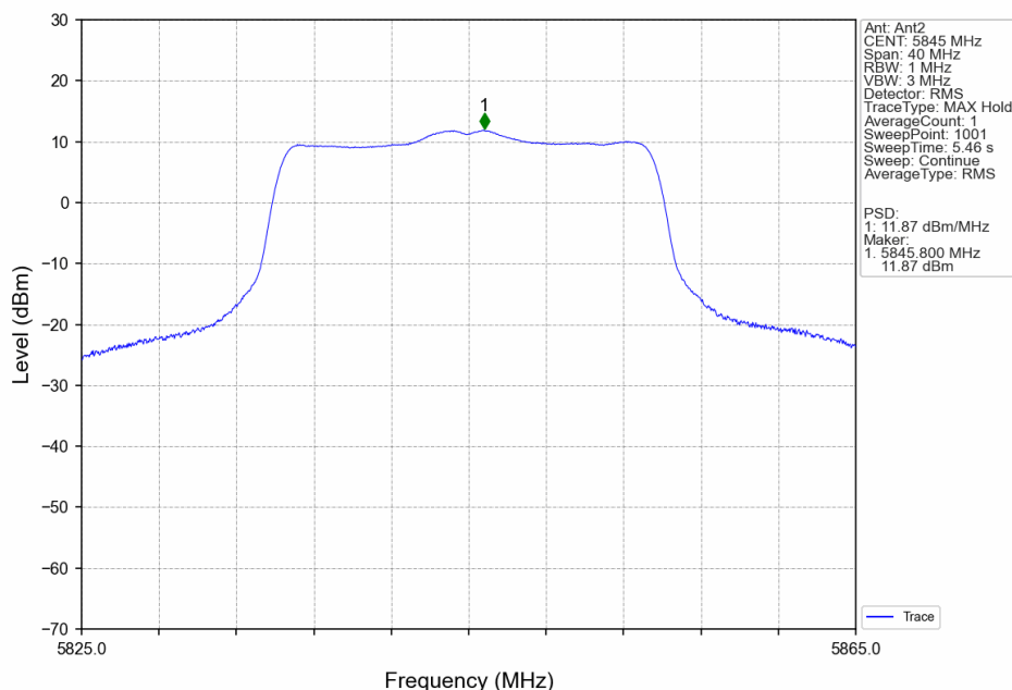
802.11ax(HEW20)_HCH_5845MHz_SU_ / _MIMO_NTNV
