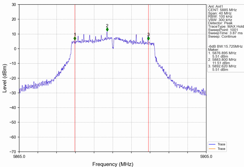
802.11ac(VHT20)_HCH_5885MHz_Ant1_NTNV
