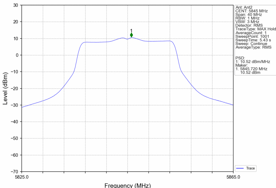
802.11n(HT20)_HCH_5845MHz_Ant2_NTNV
