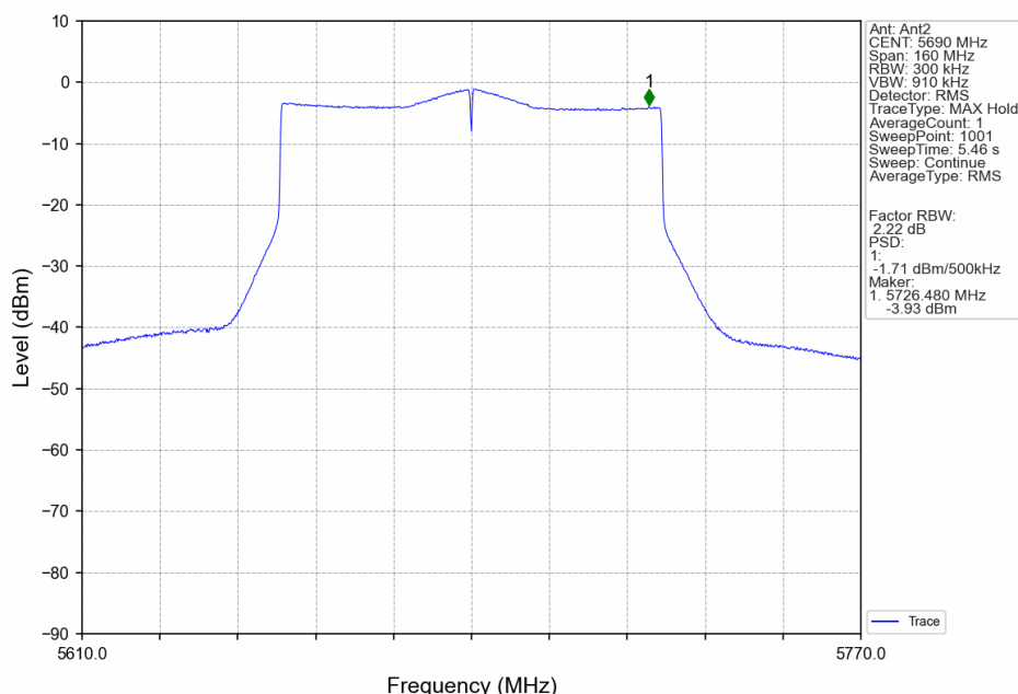
802.11ax(HEW80)_HCH_5690MHz_SU_ / _Ant2_NTNV
