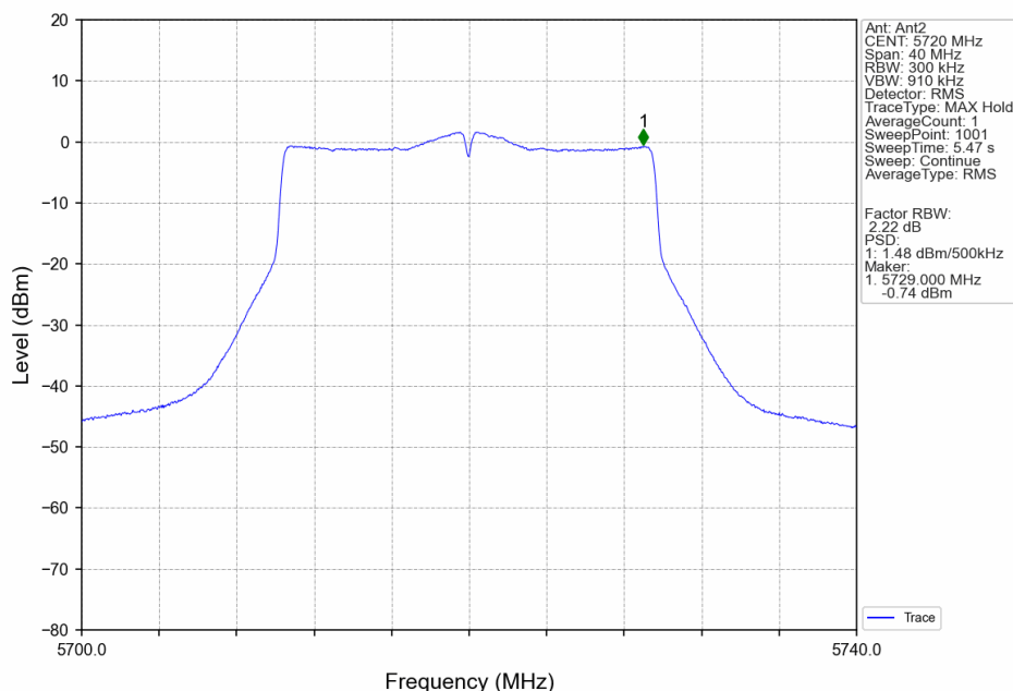
802.11ax(HEW20)_HCH_5720MHz_SU_ / _MIMO_NTNV
