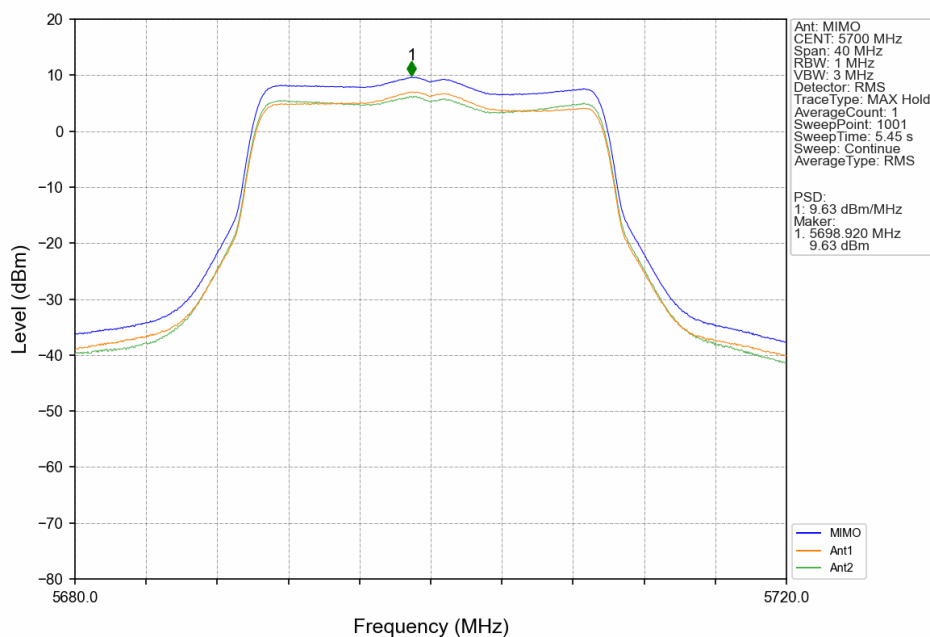
802.11ax(HEW20)_HCH_5700MHz_SU_ / _MIMO_NTNV
