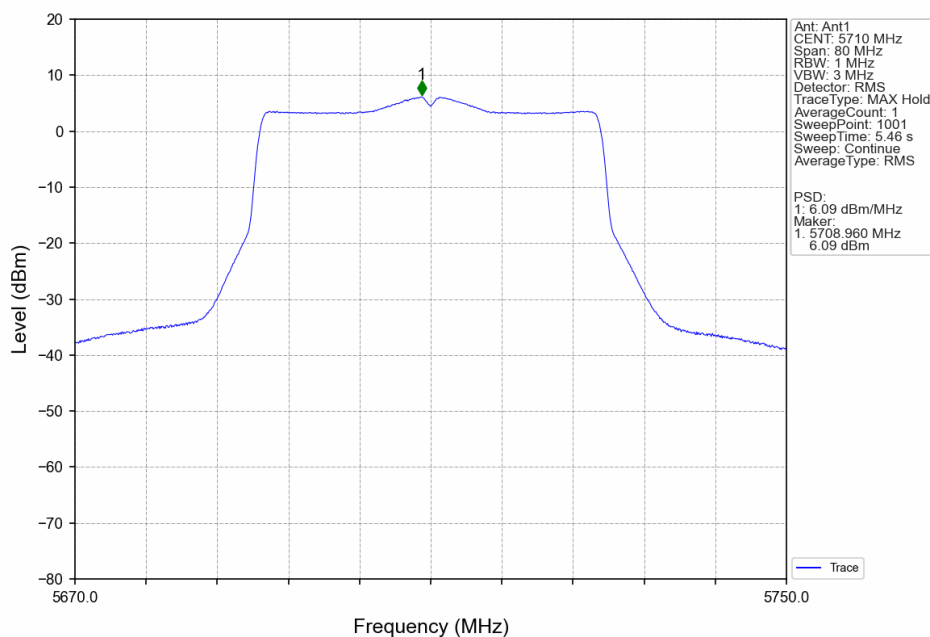
802.11ax(HEW40)_HCH_5710MHz_SU_/_Ant1_NTNV
