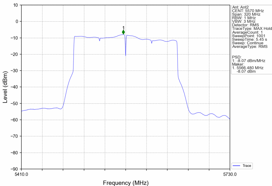
802.11ax(HEW160)_MCH_5570MHz_SU_ / _Ant2_NTNV
