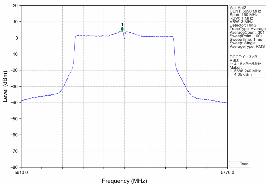
802.11ac(VHT80)_HCH_5690MHz_Ant2_NTNV
