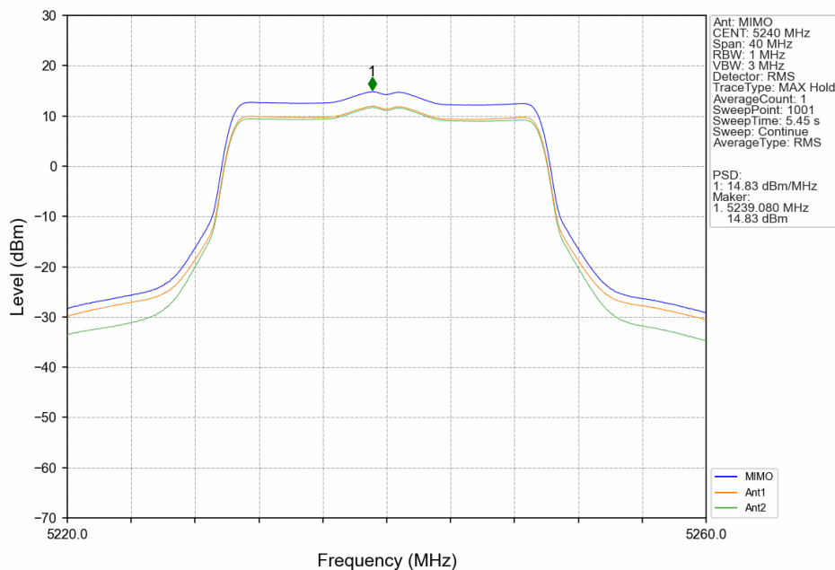
802.11ax(HEW20)_HCH_5240MHz_SU_ / _MIMO_NTNV
