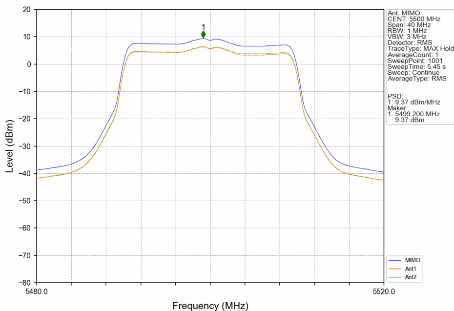
802.11ax(HEW20)_LCH_5500MHz_SU_ / _MIMO_NTNV
