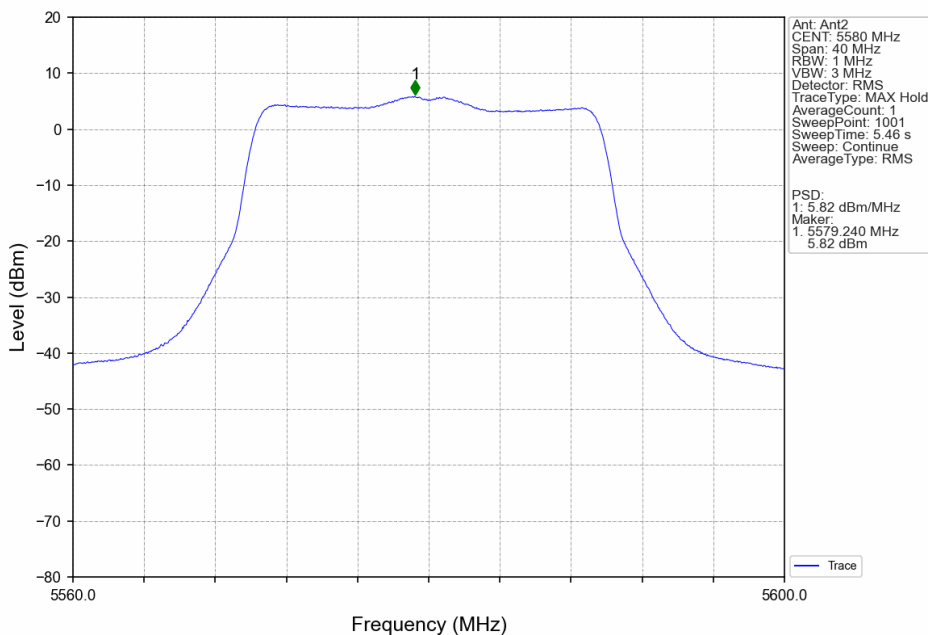
802.11ax(HEW20)_MCH_5580MHz_SU_ / _Ant2_NTNV
