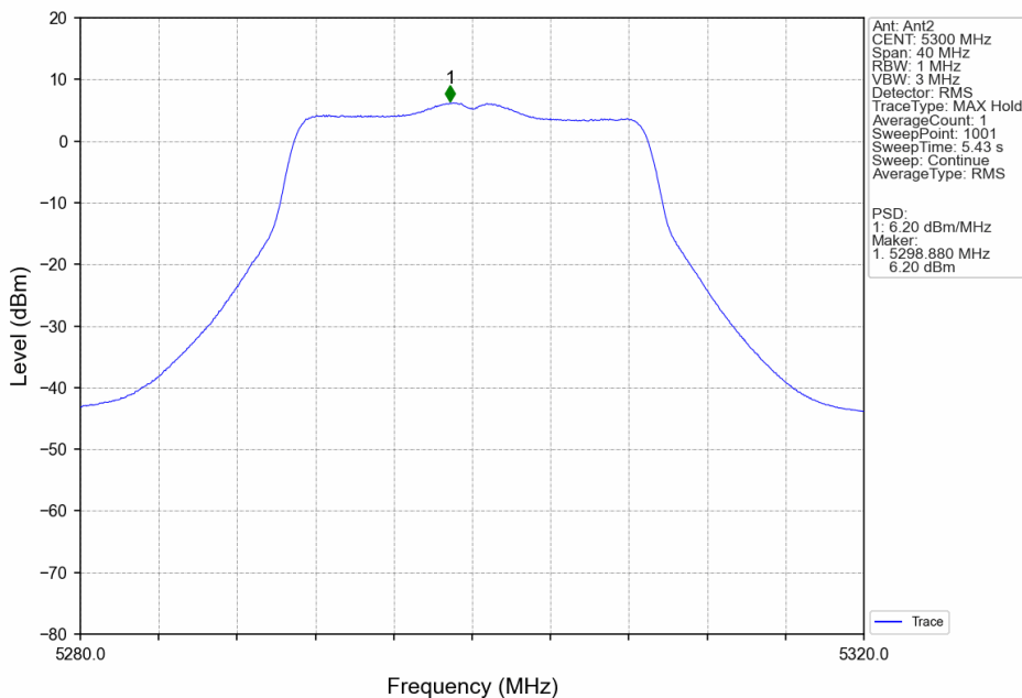
802.11ac(VHT20)_MCH_5300MHz_MIMO_NTNV
