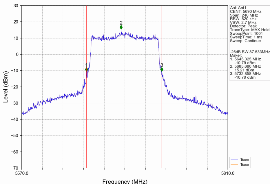
802.11ax(HEW80)_HCH_5690MHz_SU_ / _Ant1_NTNV
