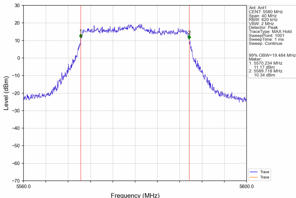
802.11ax(HEW20)_MCH_5580MHz_SU_ / _Ant1_NTNV
