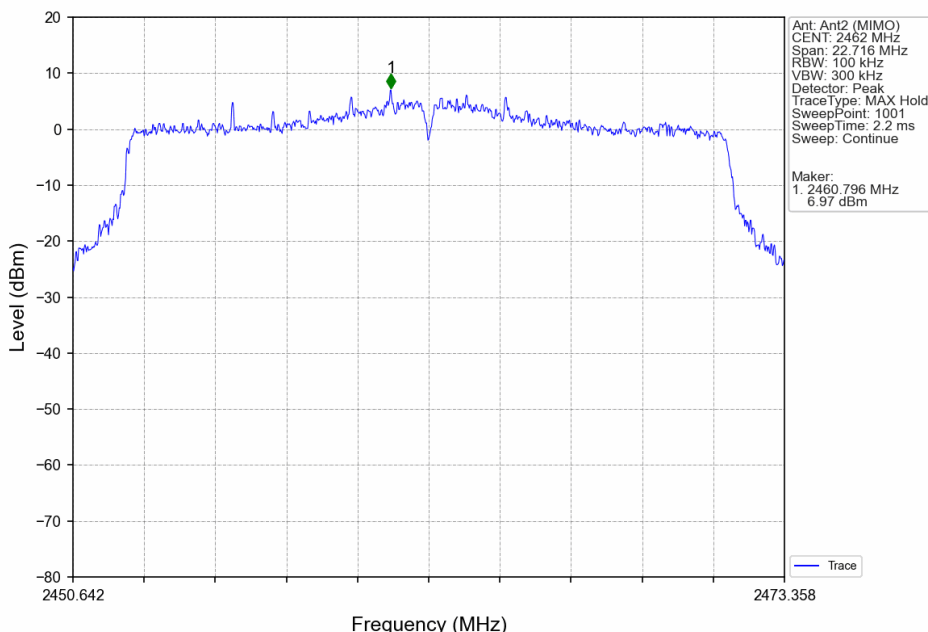
802.11ax(HEW20)_HCH_2462MHz_SU_/_Ant2 (MIMO)_NTNV
