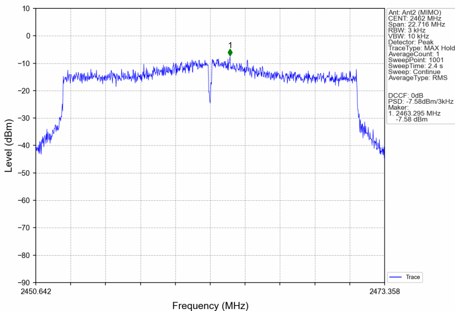
802.11ax(HEW20)_HCH_2462MHz_SU_/_Ant2 (MIMO)_NTNV
