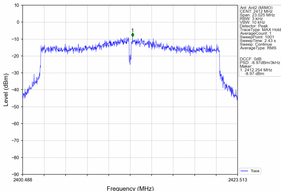
802.11ax(HEW20)_LCH_2412MHz_SU_/_Ant2 (MIMO)_NTNV
