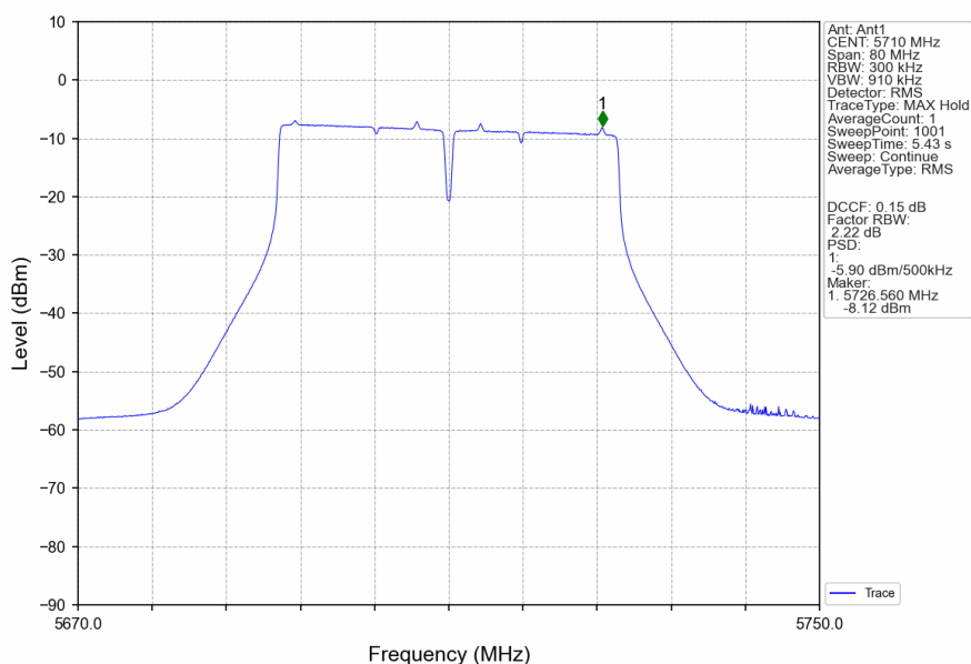
802.11ac(VHT40)_HCH_5710MHz_MIMO_NTNV
