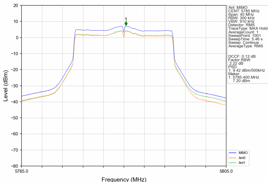
802.11ax(HEW20)_MCH_5785MHz_SU_ / _MIMO_NTNV
