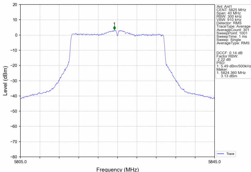
802.11ax(HEW20)_HCH_5825MHz_SU_ / _Ant1_NTNV
