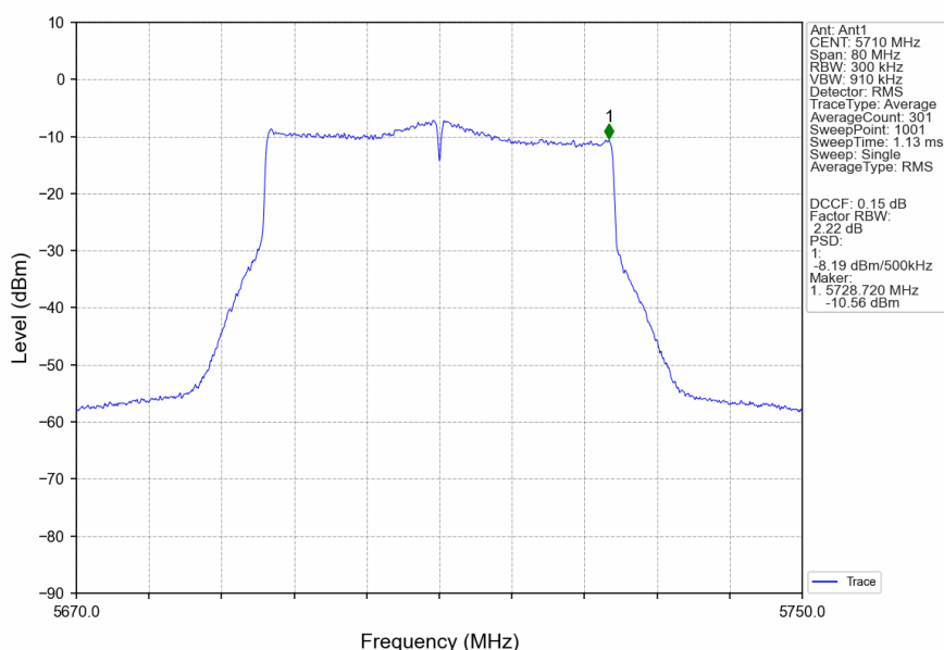
802.11ax(HEW40)_HCH_5710MHz_SU_ / _Ant1_NTNV
