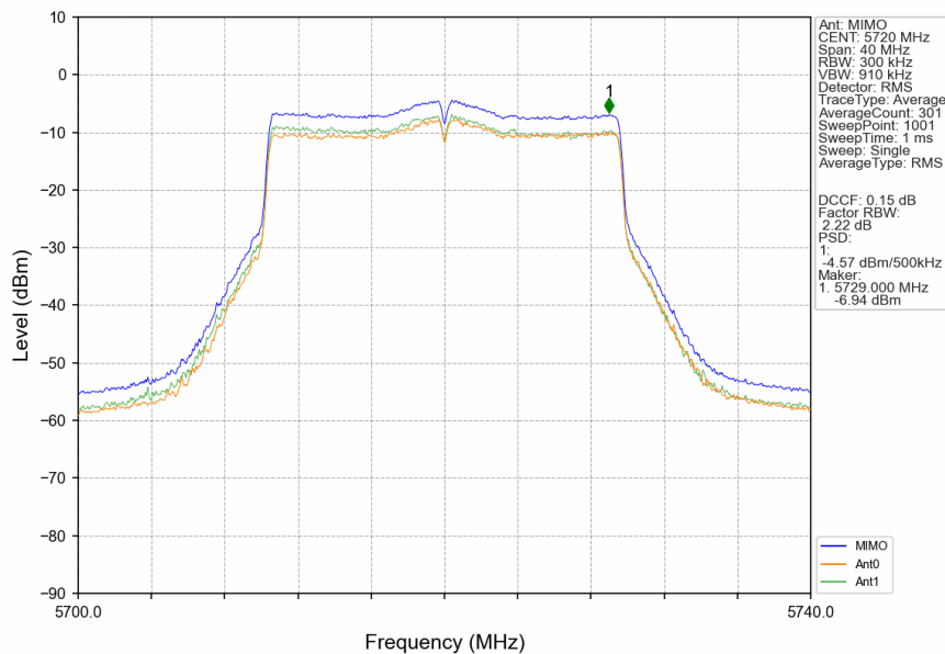
802.11ax(HEW20)_HCH_5720MHz_SU_ / _MIMO_NTNV
