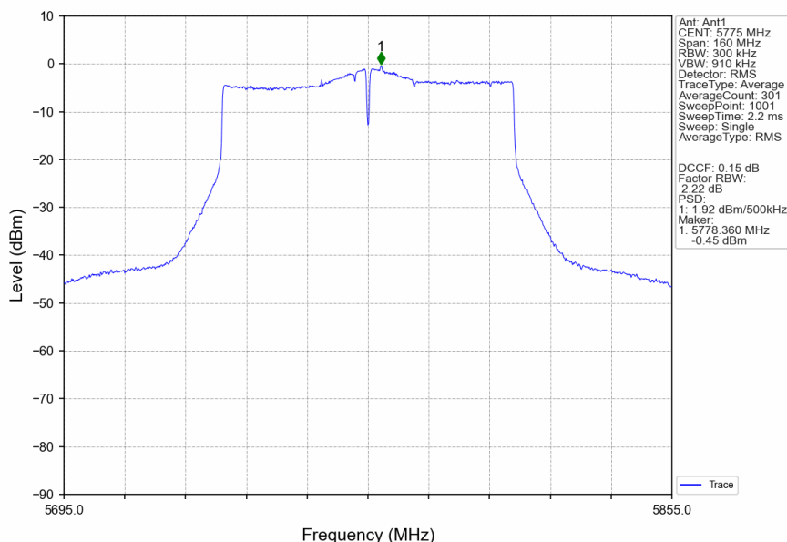
802.11ac(VHT80)_MCH_5775MHz_Ant1_NTNV
