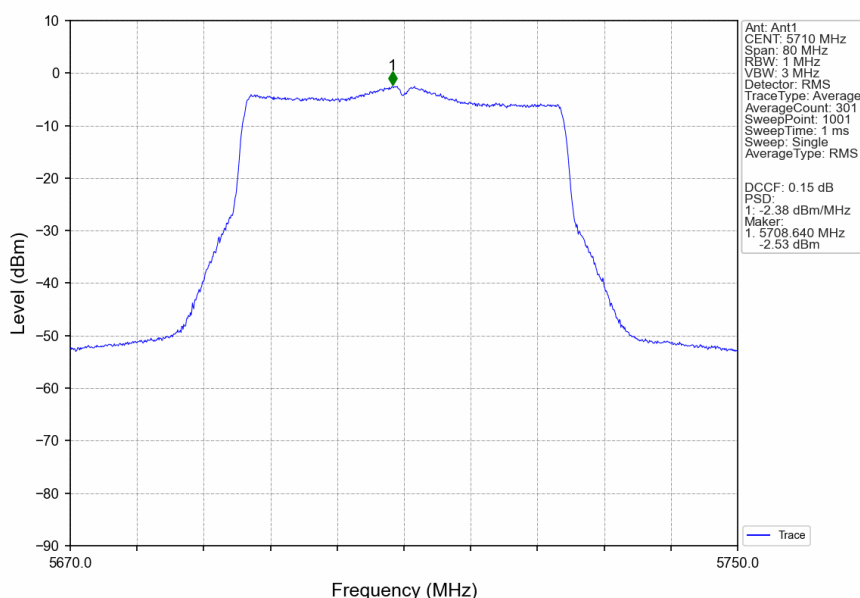
802.11ax(HEW40)_HCH_5710MHz_SU_ / _Ant1_NTNV
