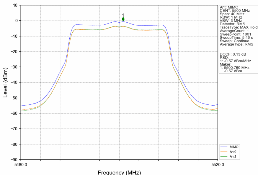
802.11ax(HEW20)_LCH_5500MHz_SU_ / _MIMO_NTNV
