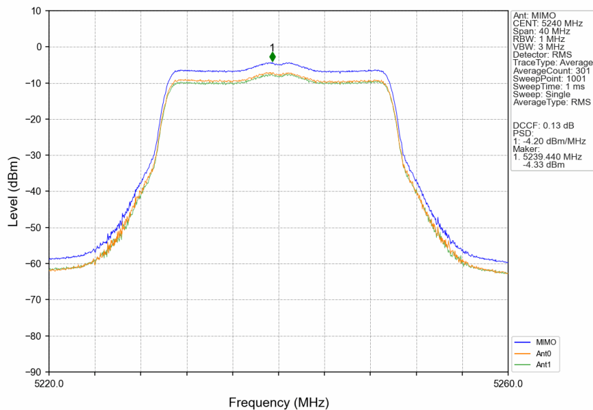
802.11ax(HEW20)_HCH_5240MHz_SU_/_MIMO_NTNV
