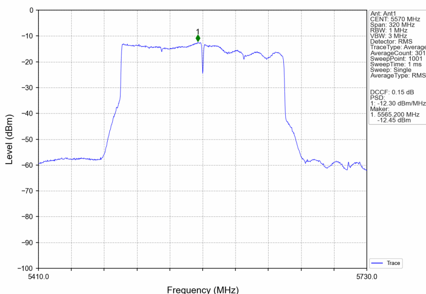
802.11ax(HEW160)_MCH_5570MHz_SU_ / _Ant1_NTNV
