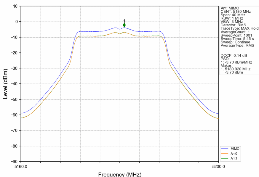
802.11ac(VHT20)_LCH_5180MHz_MIMO_NTNV
