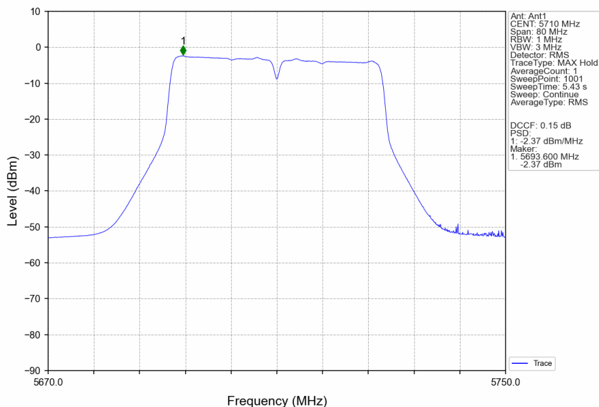
802.11ac(VHT40)_HCH_5710MHz_MIMO_NTNV
