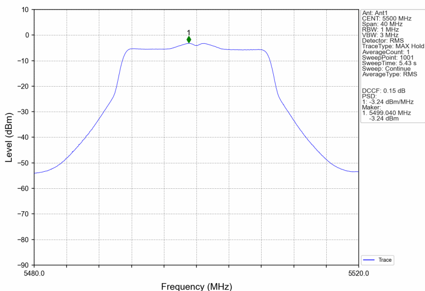
802.11ac(VHT20)_LCH_5500MHz_MIMO_NTNV
