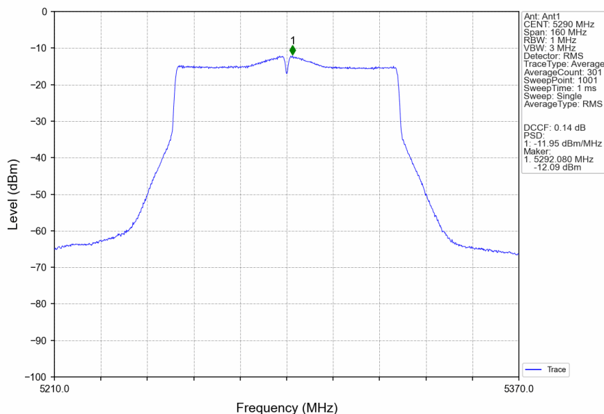
802.11ac(VHT80)_MCH_5290MHz_MIMO_NTNV
