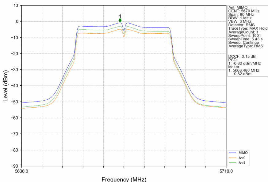
802.11n(HT40)_HCH_5670MHz_MIMO_NTNV
