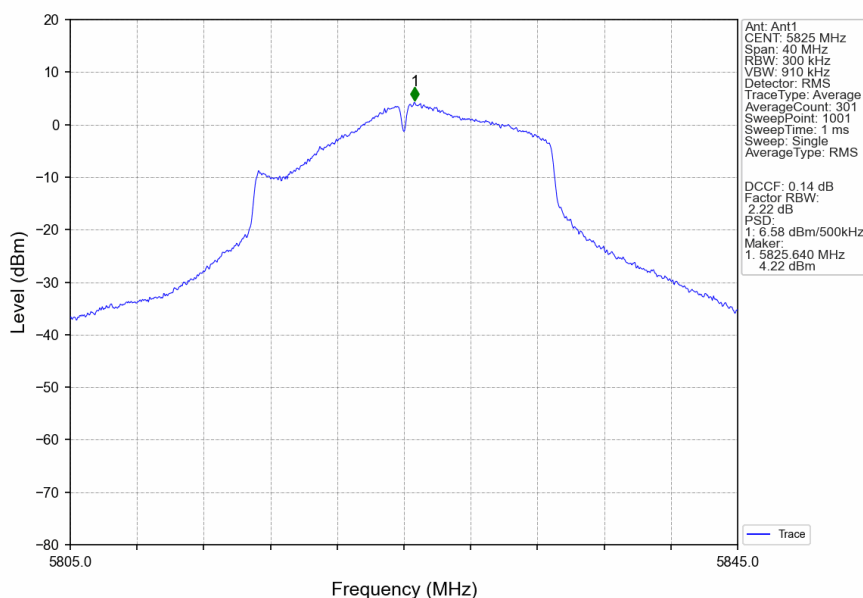
802.11ac(VHT20)_HCH_5825MHz_MIMO_NTNV
