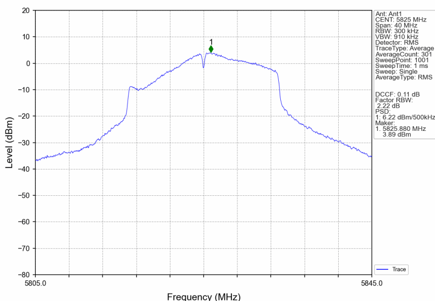
02.11n(HT20)_HCH_5825MHz_Ant1_NTNV
