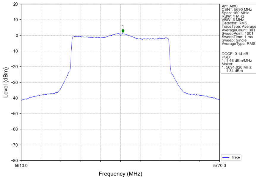
802.11ax(HEW80)_HCH_5690MHz_SU_/_Ant0_NTNV
