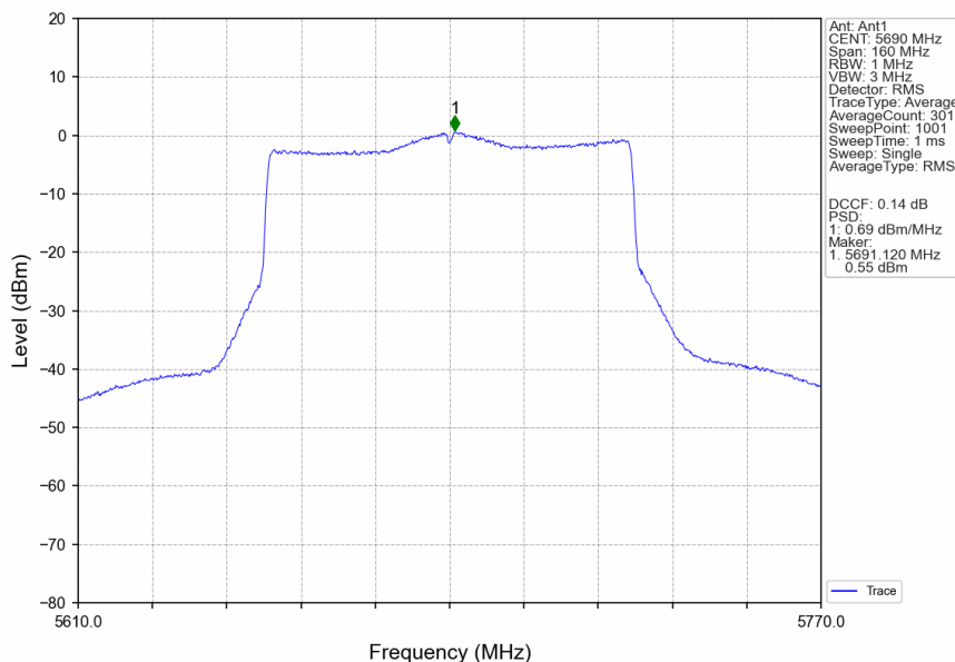
802.11ax(HEW80)_HCH_5690MHz_SU_ / _MIMO_NTNV
