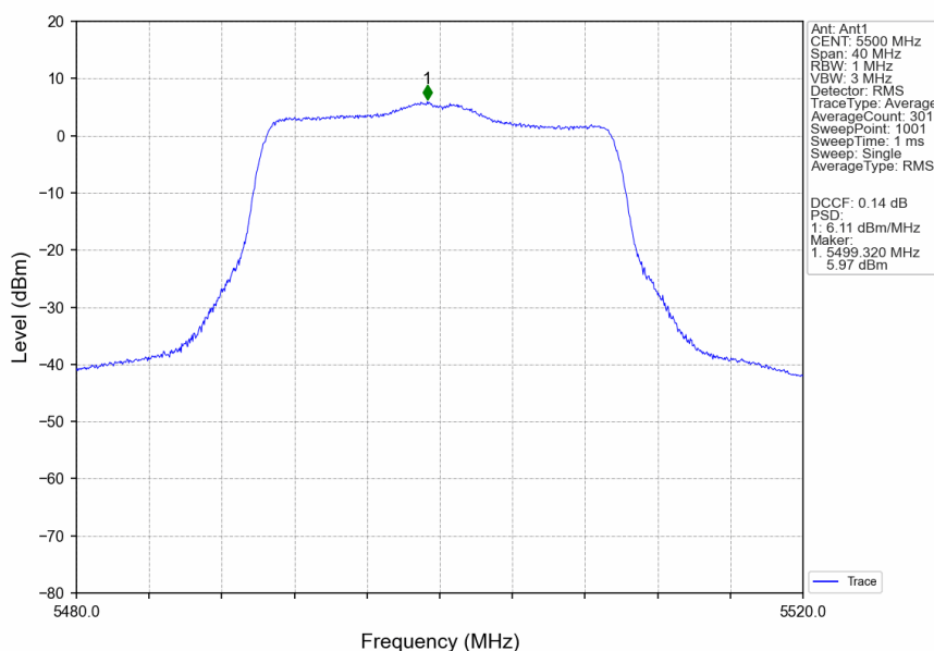
802.11ax(HEW20)_LCH_5500MHz_SU_ / _MIMO_NTNV
