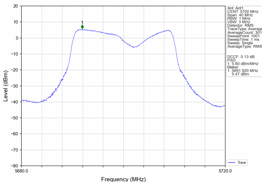
802.11ax(HEW20)_HCH_5700MHz_SU_/_MIMO_NTNV
