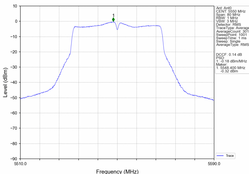
802.11ac(VHT40)_MCH_5550MHz_Ant0_NTNV
