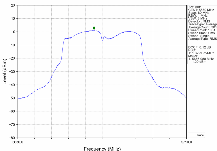
802.11n(HT40)_HCH_5670MHz_Ant1_NTNV
