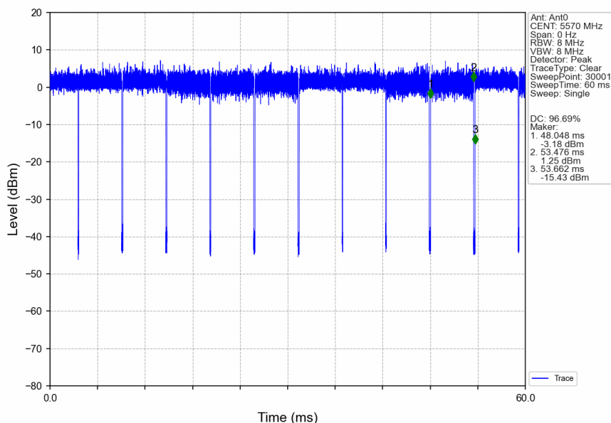
802.11ac(VHT160)_MCH_5570MHz_Ant0_NTNV
