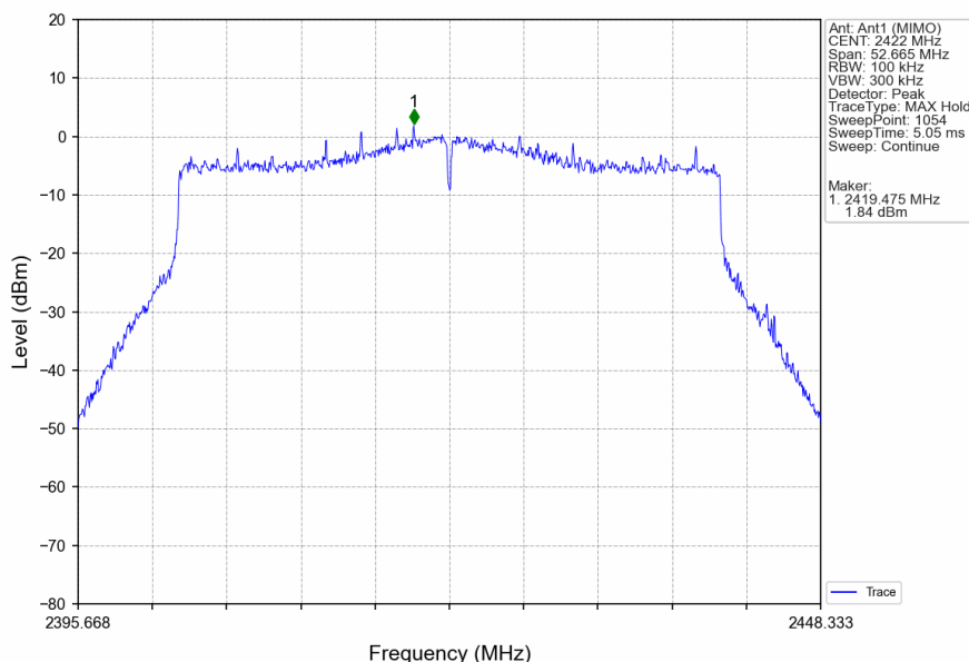
802.11ax(HEW40)_LCH_2422MHz_SU_/_Ant1 (MIMO)_NTNV
