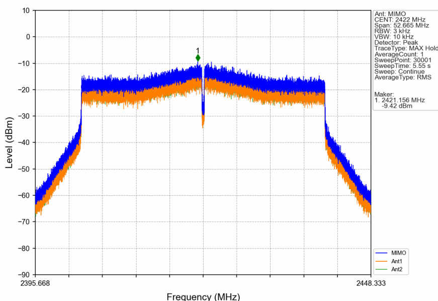
802.11ax(HEW40)_LCH_2422MHz_SU_/_MIMO_NTNV
