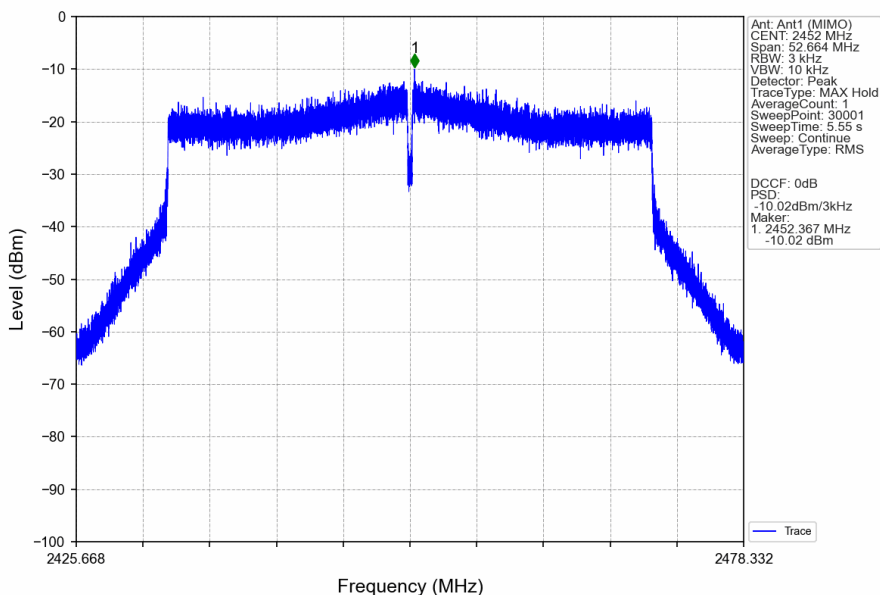
802.11ax(HEW40)_HCH_2452MHz_SU_/_MIMO_NTNV
