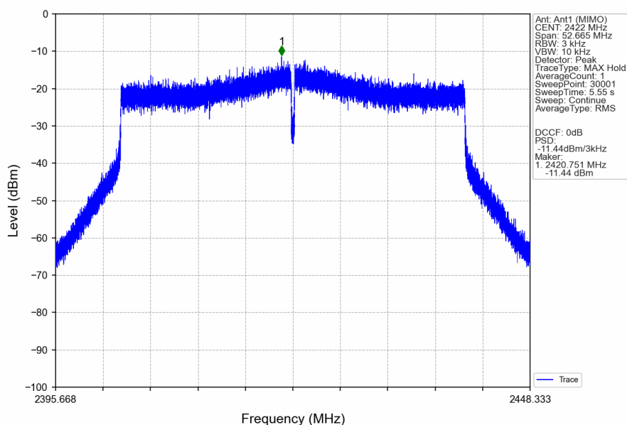
802.11ax(HEW40)_LCH_2422MHz_SU_/_MIMO_NTNV
