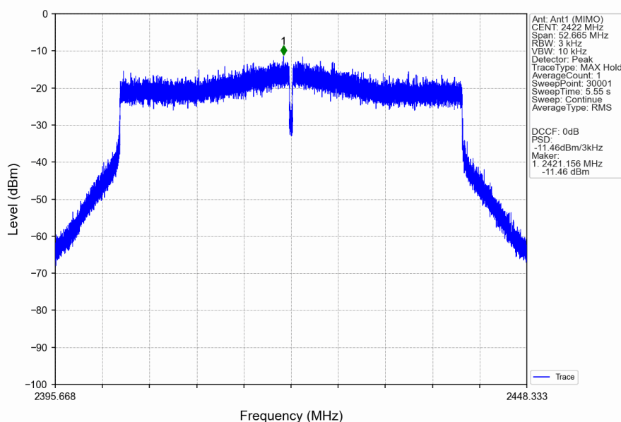
802.11ax(HEW40)_LCH_2422MHz_SU_/_MIMO_NTNV
